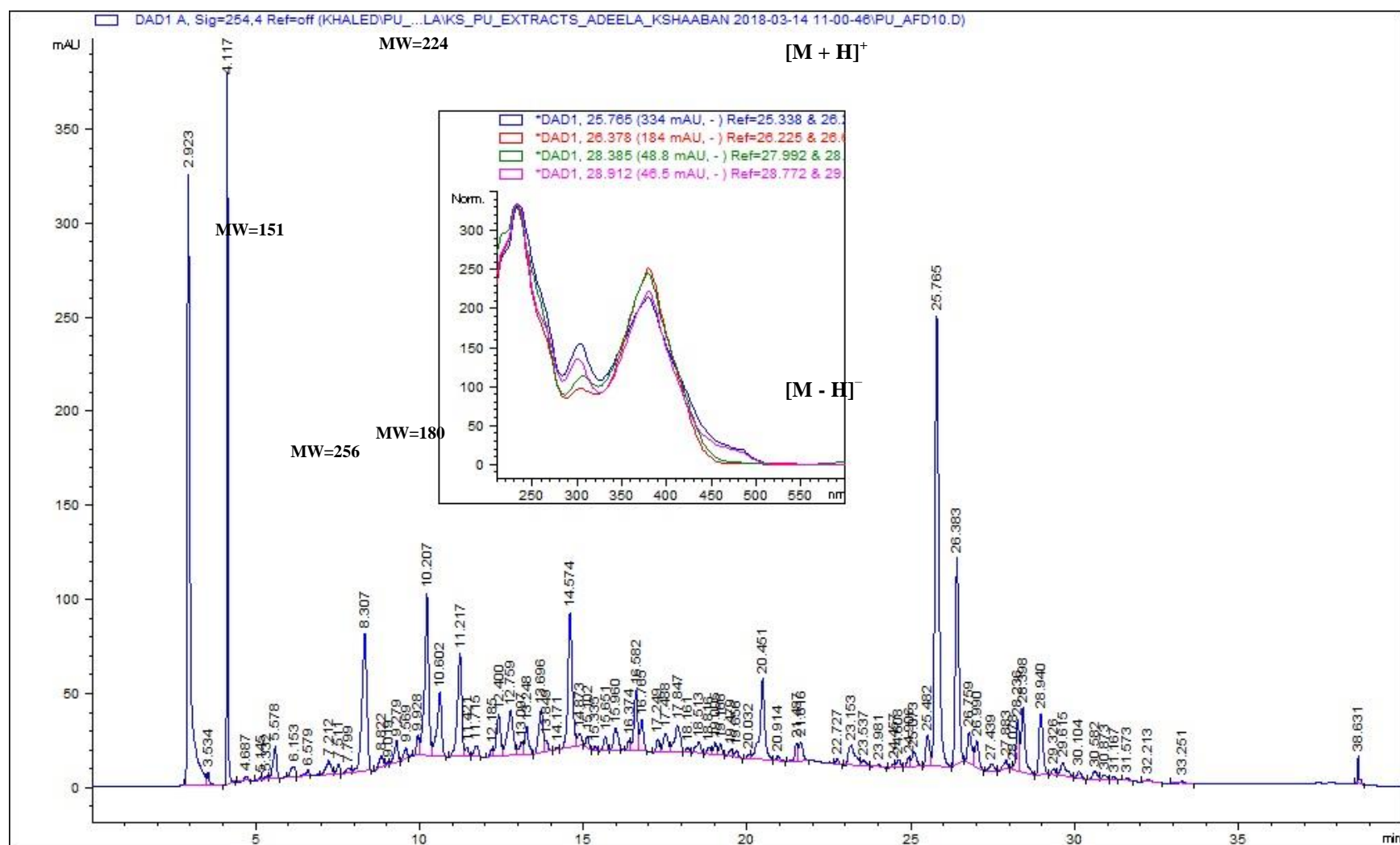
Figure S11. HPLC/UV analyses of AFD10 crude extract. HPLC-conditions: Detection wavelength 254 nm; solvent A: H 2 O/0.1% TFA; solvent B: acetonitrile; flow rate: 1.0 mL min -1 ; 0-30 min, 95-0% A (linear gradient); 30-35 min 0% A; 35-36 min 0-95% A (linear gradient); 36-40 min 95% A.
