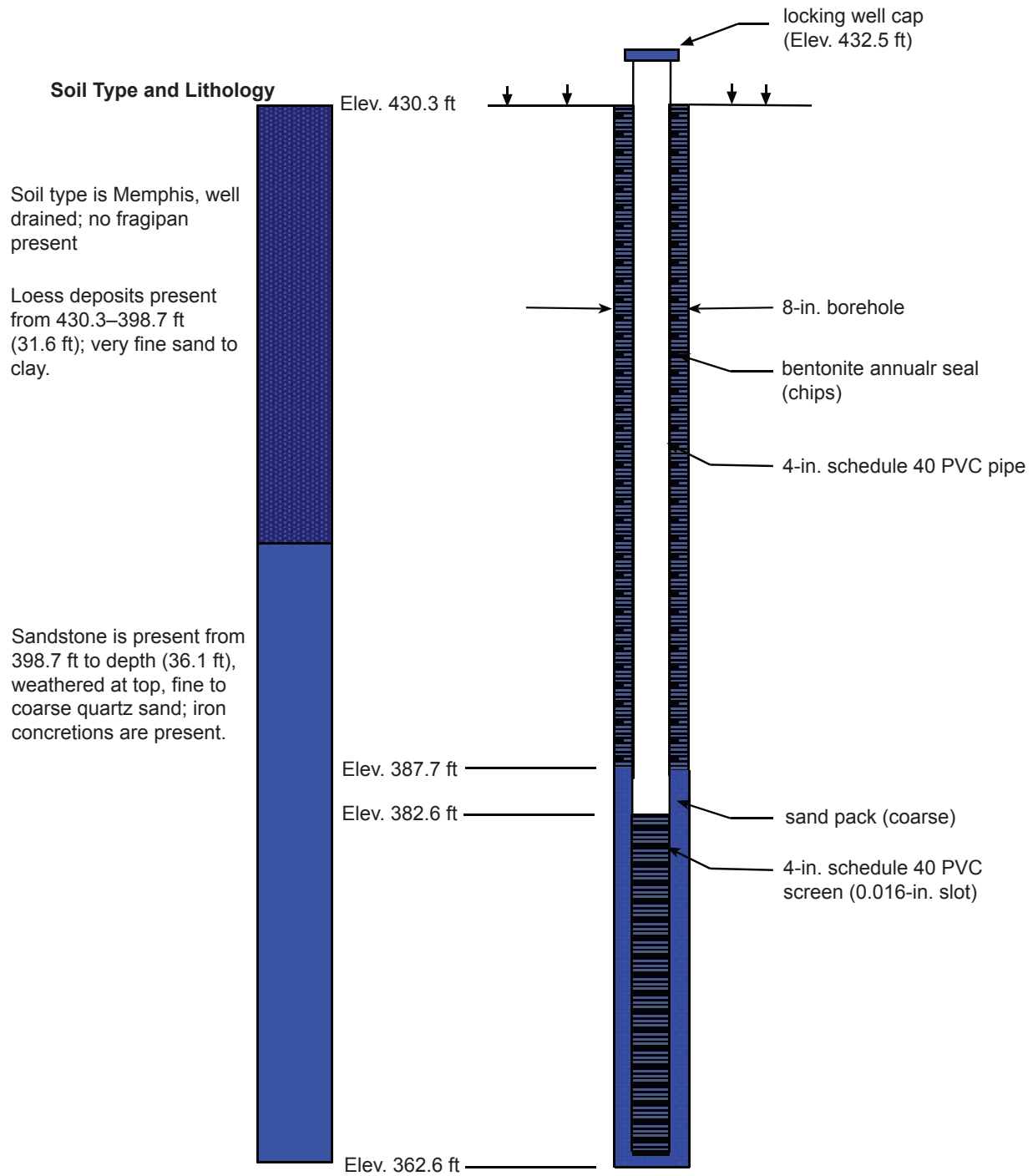
Domestic Well 12 (DW12) Diagram not to scale
