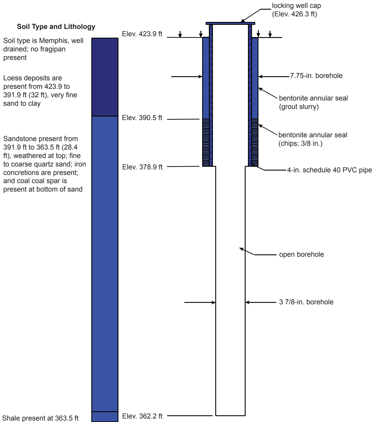
Domestic Well 7 (DW07) Diagram not to scale
