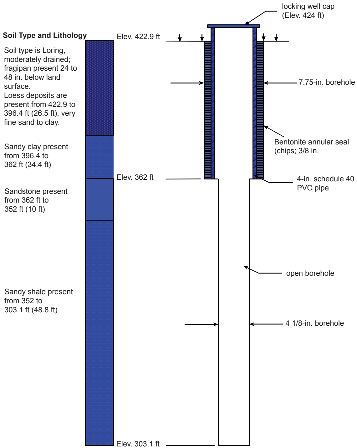
Domestic Well 6 (DW06) Diagram not to scale
