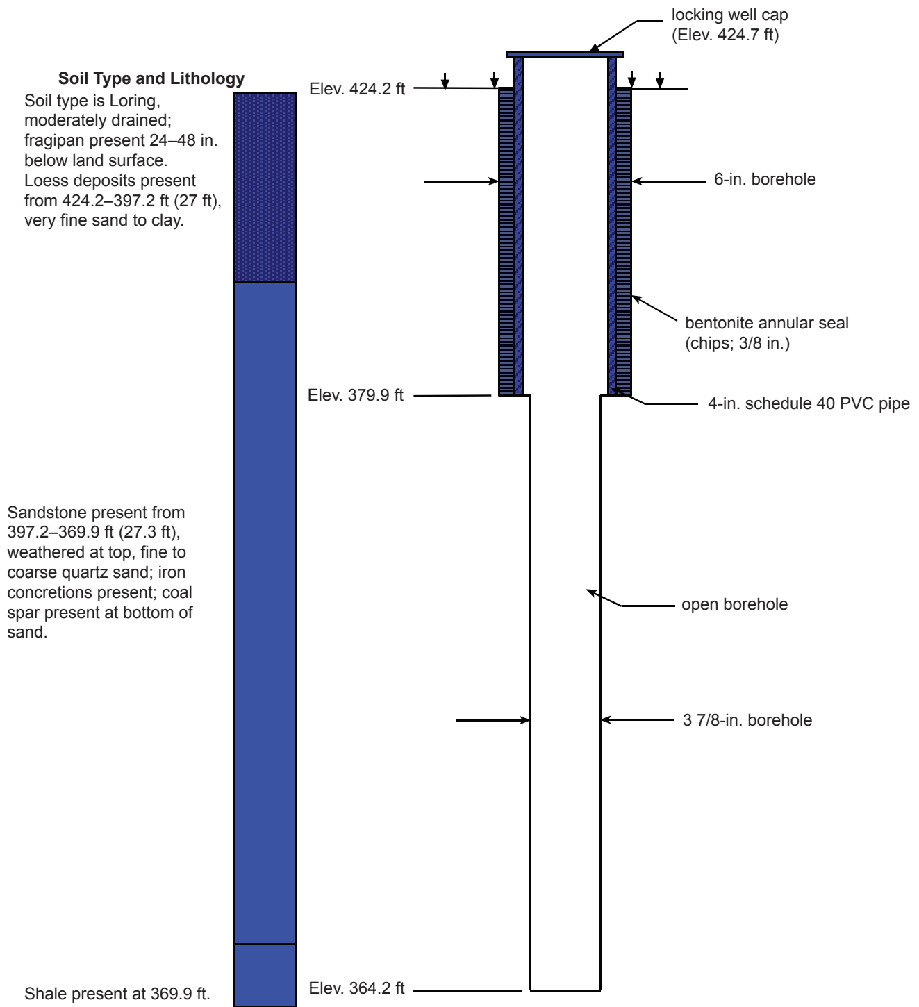
Domestic Well 8 (DW08) Diagram not to scale
