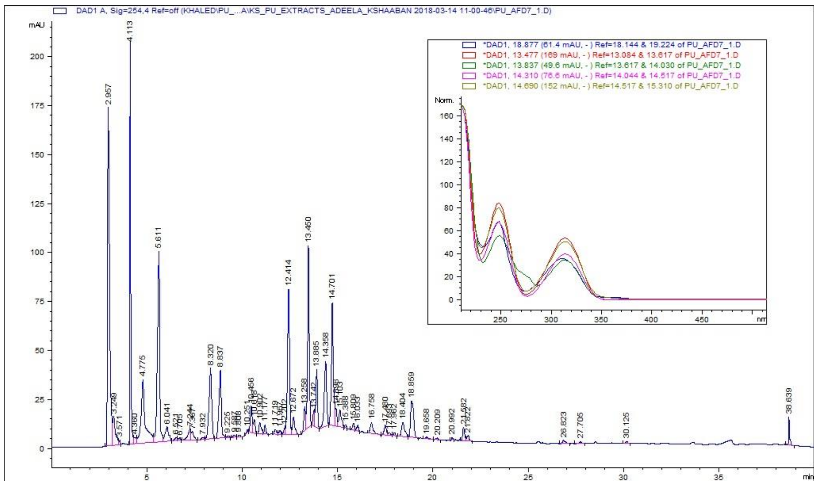
Figure S7. HPLC/UV analyses of AFD7 crude extract. HPLC-conditions: Detection wavelength 254 nm; solvent A: H 2 O/0.1% TFA; solvent B: acetonitrile; flow rate: 1.0 mL min -1 ; 0-30 min, 95-0% A (linear gradient); 30-35 min 0% A; 35-36 min 0-95% A (linear gradient); 36-40 min 95% A.
