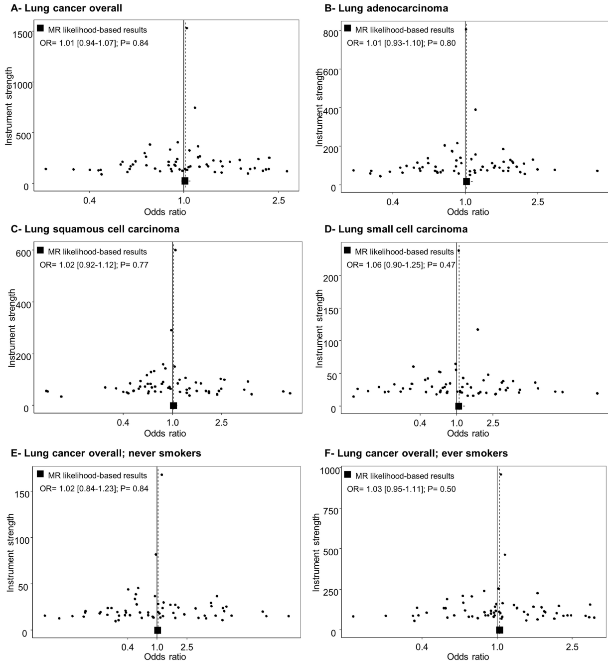
S6 Fig - Funnel plots for the distribution of risk estimates of HDL instrumental common SNPs along with MR causal effect lung cancer subtypes. OR: Odds ratio; Int: Intercept; P: P value.
