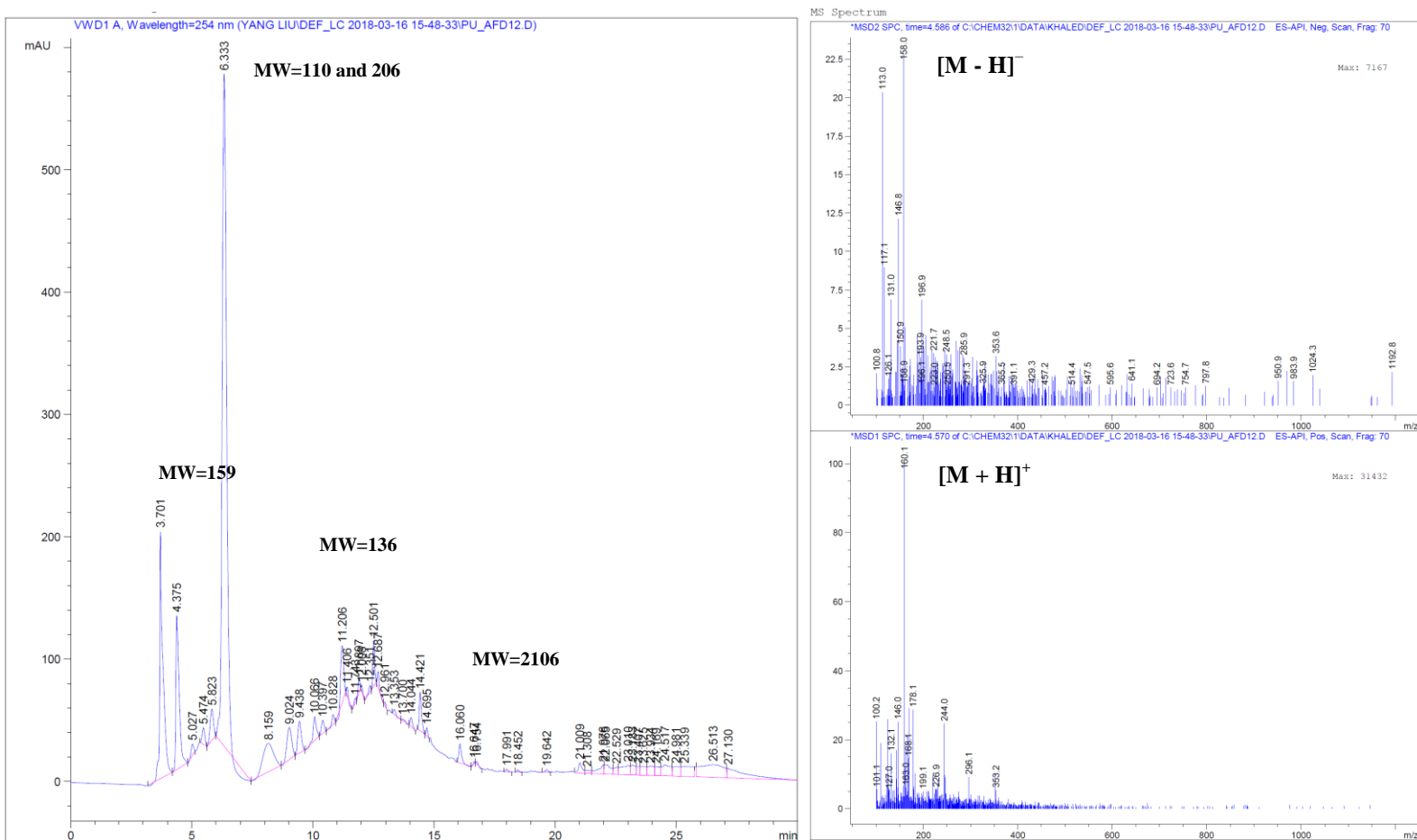
Figure S14. HPLC/MS analyses of AFD12 crude extract. HPLC-conditions: Detection wavelength 254 nm; solvent A: H 2 O/0.1% Formic acid, solvent B: CH 3 CN/0.1% Formic acid; flow rate: 0.5 mL min -1 ; 0-4 min, 10% B; 4-22 min, 10-100% B; 22-27 min, 100% B; 27-29 min, 100%-10% B; 29-30 min, 10 % B. (MW = Molecular Weight)
