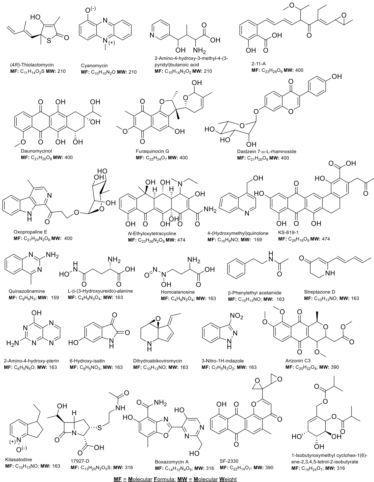
Figure S20: Chemical structures of the suggested Streptomyces metabolites based on HPLC-UV/Vis and LC-MS analyses and by searching in AntiBase 2017.
