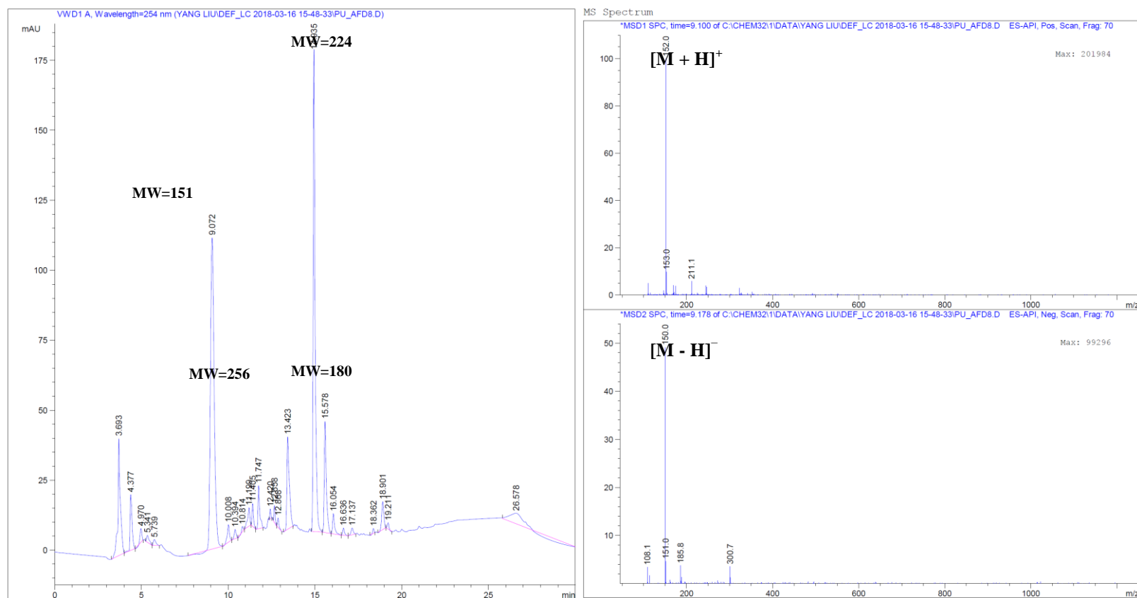
Figure S10. HPLC/MS analyses of AFD8 crude extract. HPLC-conditions: Detection wavelength 254 nm; solvent A: H 2 O/0.1% Formic acid, solvent B: CH 3 CN/0.1% Formic acid; flow rate: 0.5 mL min -1 ; 0-4 min, 10% B; 4-22 min, 10-100% B; 22-27 min, 100% B; 27-29 min, 100%-10% B; 29-30 min, 10% B. (MW = Molecular Weight)
