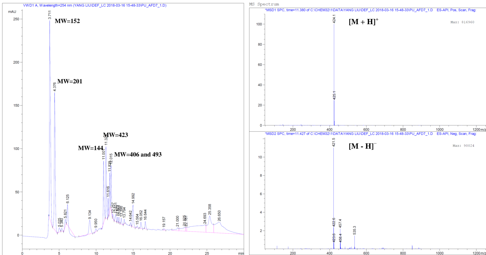
Figure S8. HPLC/MS analyses of AFD7 crude extract. HPLC-conditions: Detection wavelength 254 nm; solvent A: H 2 O/0.1% Formic acid, solvent B: CH 3 CN/0.1% Formic acid; flow rate: 0.5 mL min -1 ; 0-4 min, 10% B; 4-22 min, 10-100% B; 22-27 min, 100% B; 27-29 min, 100%-10% B; 29-30 min, 10 % B. (MW = Molecular Weight)
