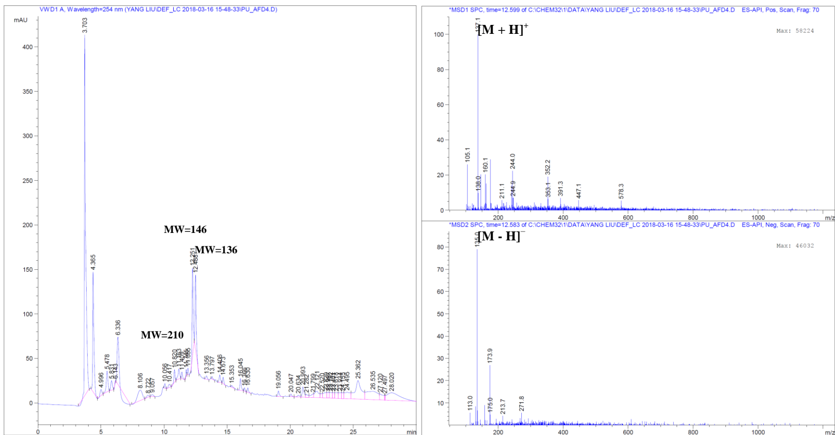
Figure S6. HPLC/MS analyses of AFD4 crude extract. HPLC-conditions: Detection wavelength 254 nm; solvent A: H 2 O/0.1% Formic acid, solvent B: CH 3 CN/0.1% Formic acid; flow rate: 0.5 mL min -1 ; 0-4 min, 10% B; 4-22 min, 10-100% B; 22-27 min, 100% B; 27-29 min, 100%-10% B; 29-30 min, 10% B. (MW = Molecular Weight)
