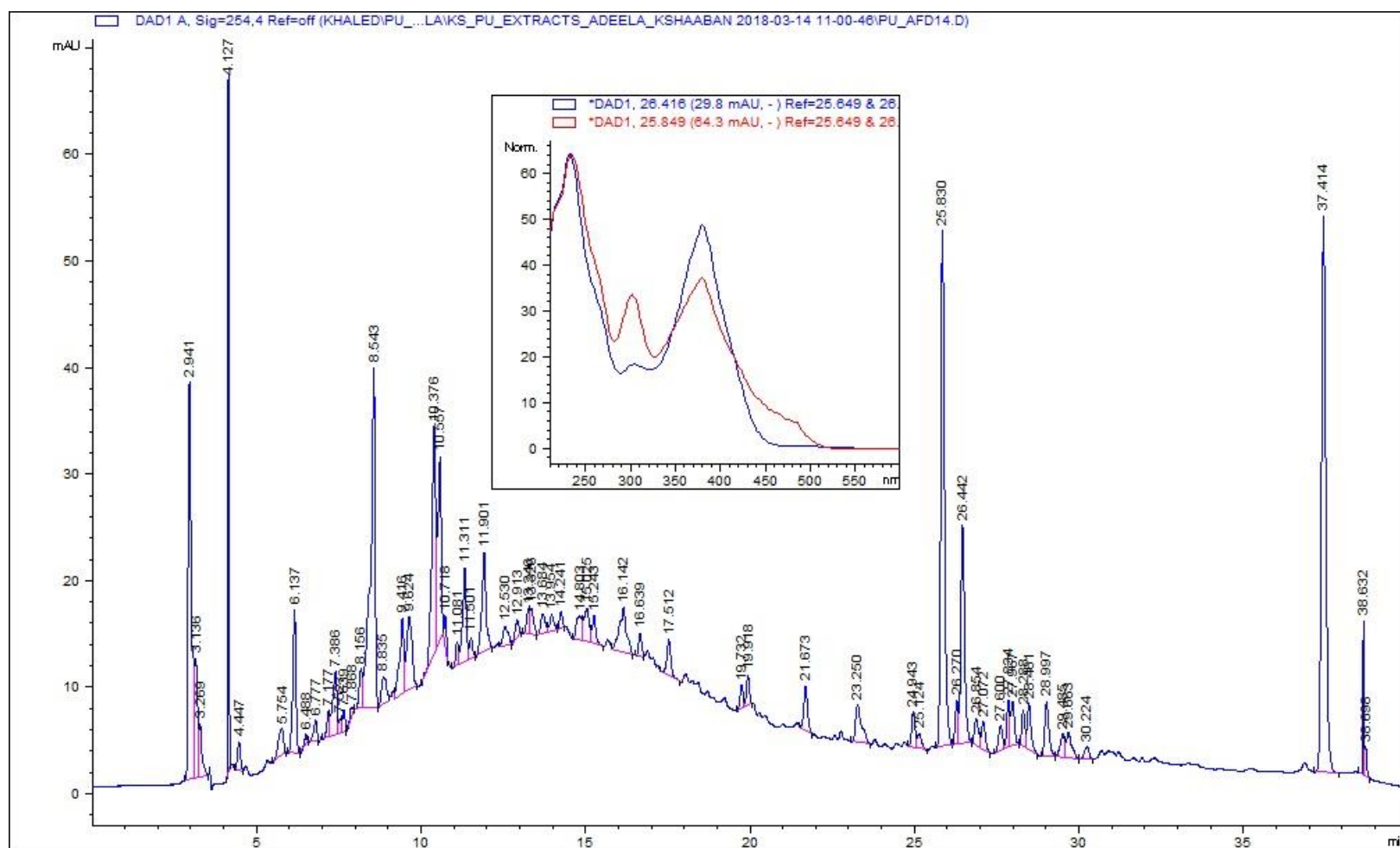
Figure S15. HPLC/UV analyses of AFD14 crude extract. HPLC-conditions: Detection wavelength 254 nm; solvent A: H 2 O/0.1% TFA; solvent B: acetonitrile; flow rate: 1.0 mL min -1 ; 0-30 min, 95-0% A (linear gradient); 30-35 min 0% A; 35-36 min 0-95% A (linear gradient); 36-40 min 95% A.
