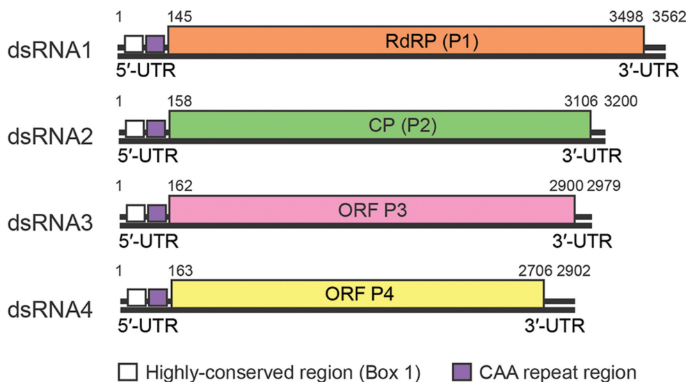
Fig. 2. Genome organization of Penicillium chrysogenum virus isolate ATCC 9480 (PcV-ATCC9480). The genome consists of four dsRNA segments, each of which is monocistronic. The RdRP (P1) ORF (nt positions 145–3498 on dsRNA1), the CP (P2) ORF (nt positions 158–3106 on dsRNA2), the P3 ORF (nt positions 162–2900 on dsRNA3) and the P4 ORF (nt positions 163–2706 on dsRNA4) are represented by rectangular boxes.
