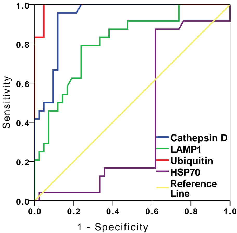
Figure e-1. Receiver Operator Characteristic (ROC) curve for classification of cross-sectional patients with AD, as contrasted with matched controls (AC) based on measured levels of individual exosomal proteins and discriminant scores calculated from a stepwise model.
