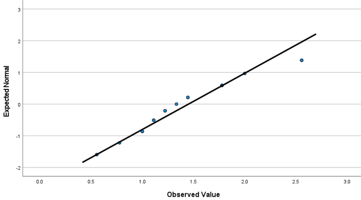
Normal Q-Q Plot of Post MCOP2 Teacher Facilitation Mean
