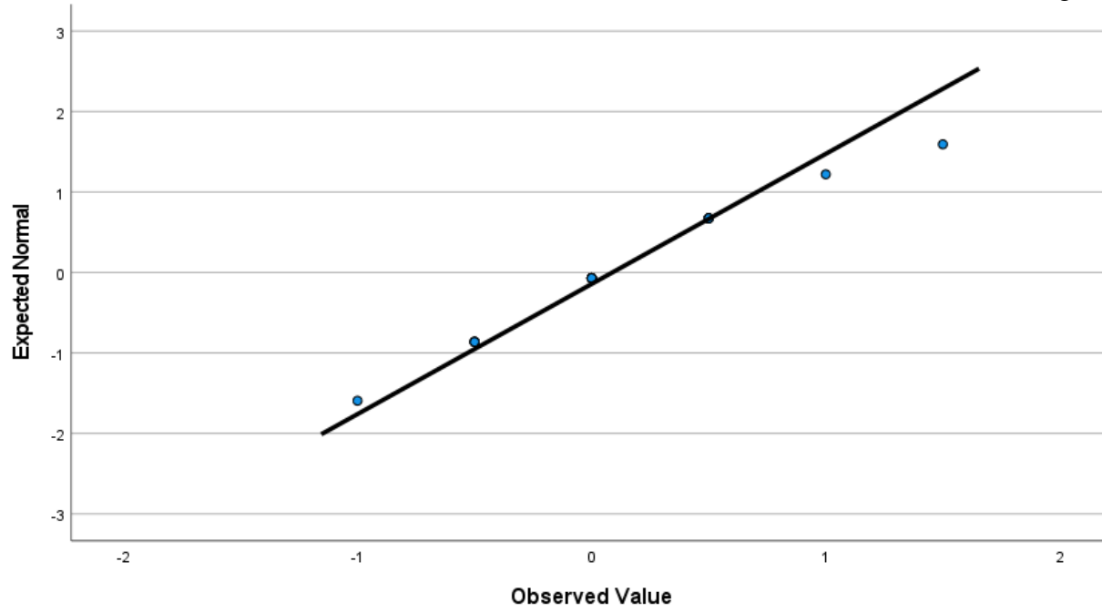
Normal Q-Q Plot of GainTPACKOC (Gain TPACK Overarching Concept)
