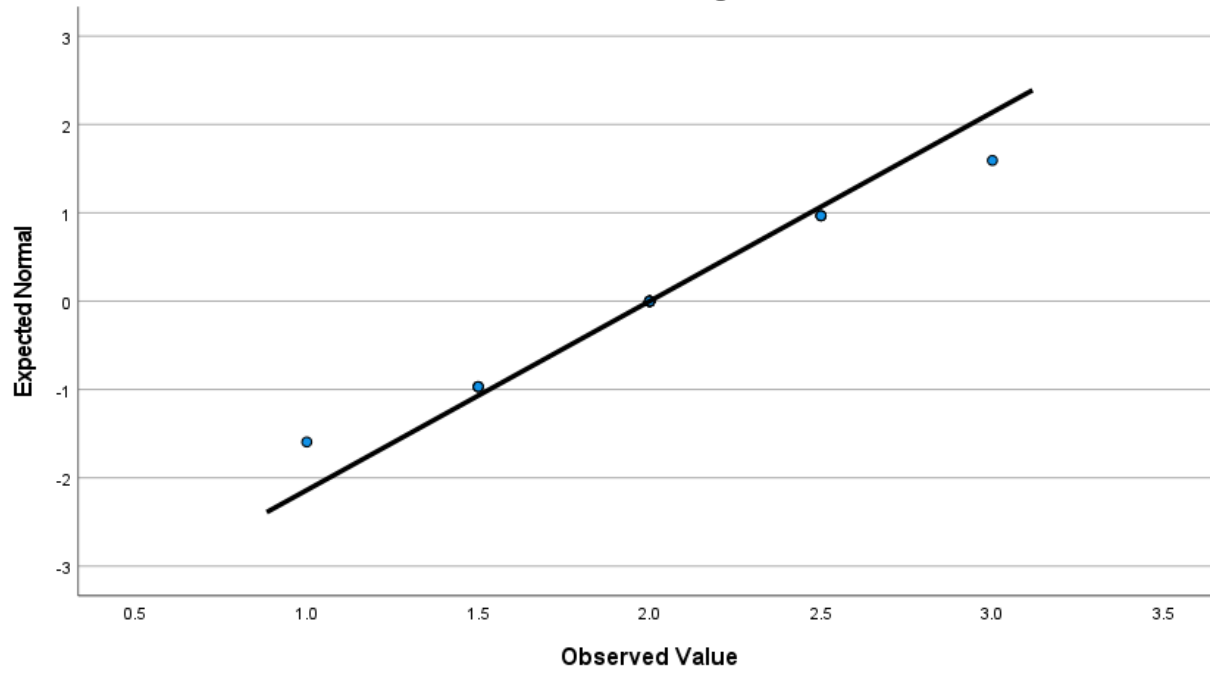
Normal Q-Q Plot of Post Knowledge of Students
