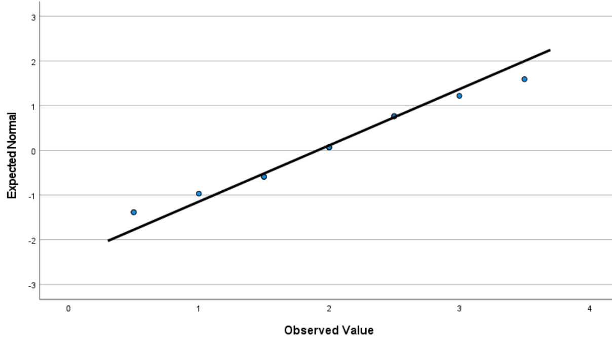
Normal Q-Q Plot of Pre Instructional Strategies
