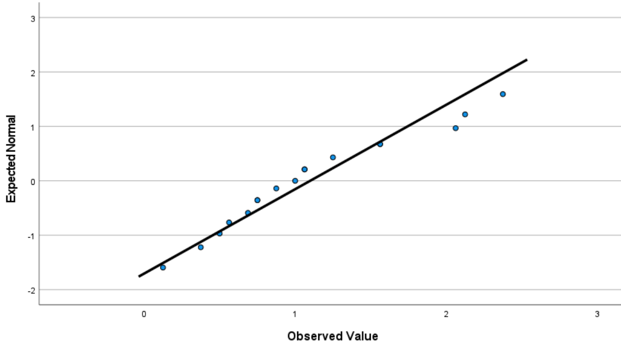
Normal Q-Q Plot of Pre MCOP2 Total Mean (Pre-MCOP 2 Overall Mean)
