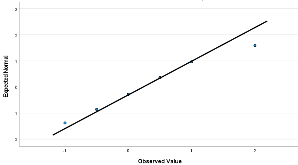
Normal Q-Q Plot of GainTPACKIS (Gain TPACK Instructional Strategies)
