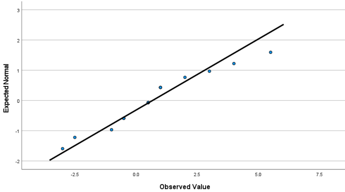
Normal Q-Q Plot of GainTPACK (Gain TPACK Overall Mean)
