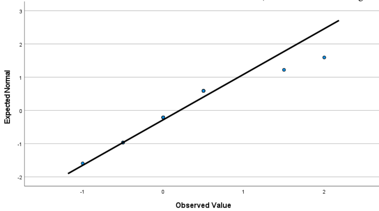
Normal Q-Q Plot of GainTPACKKoC (Gain TPACK Knowledge of Curriculum)
