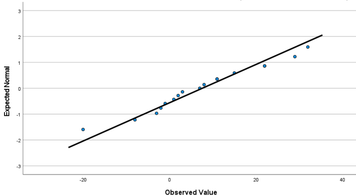
Normal Q-Q Plot of GainMCOP2 (Gain MCOP 2 Overall Mean)
