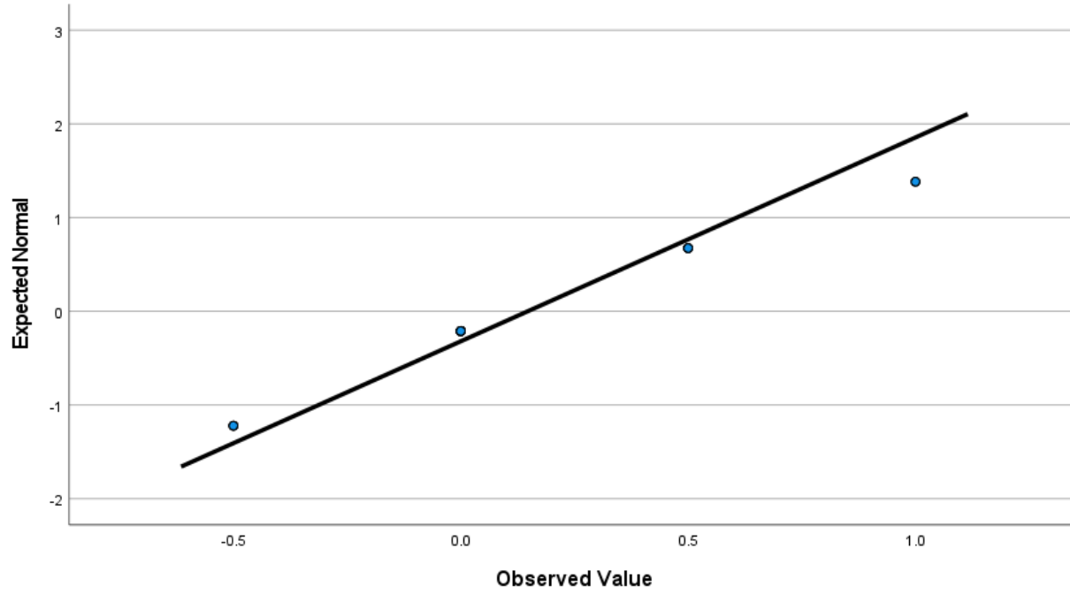
Normal Q-Q Plot of GainTPACKKoS (Gain TPACK Knowledge of Students)
