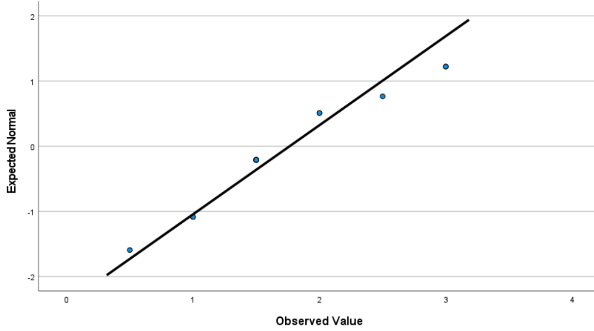
Normal Q-Q Plot of Pre Knowledge of Curriculum
