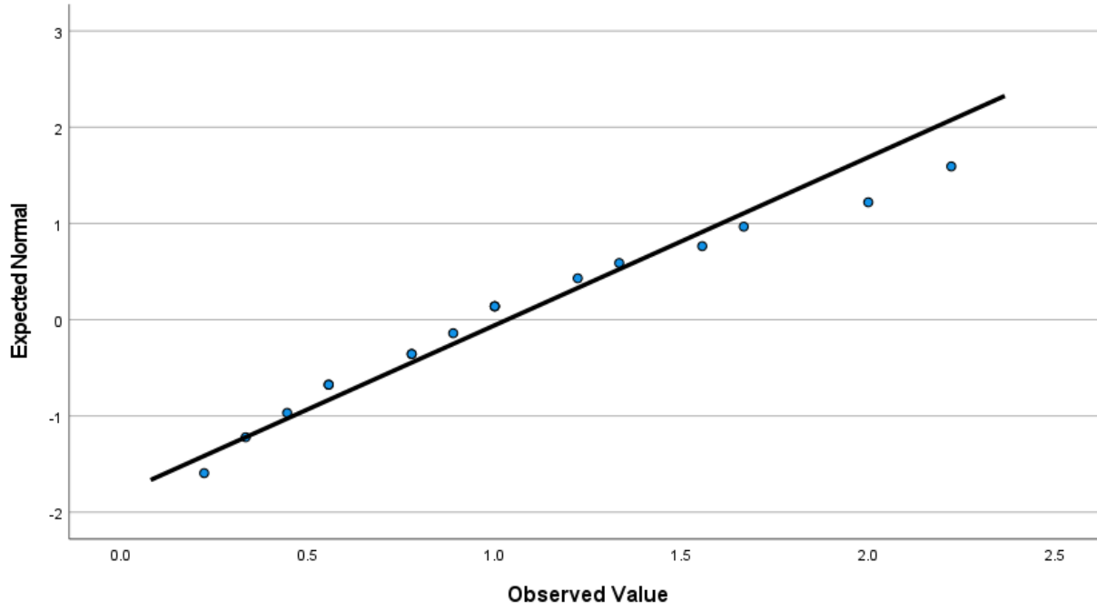
Normal Q-Q Plot of Pre MCOP2 Teacher Facilitation Mean
