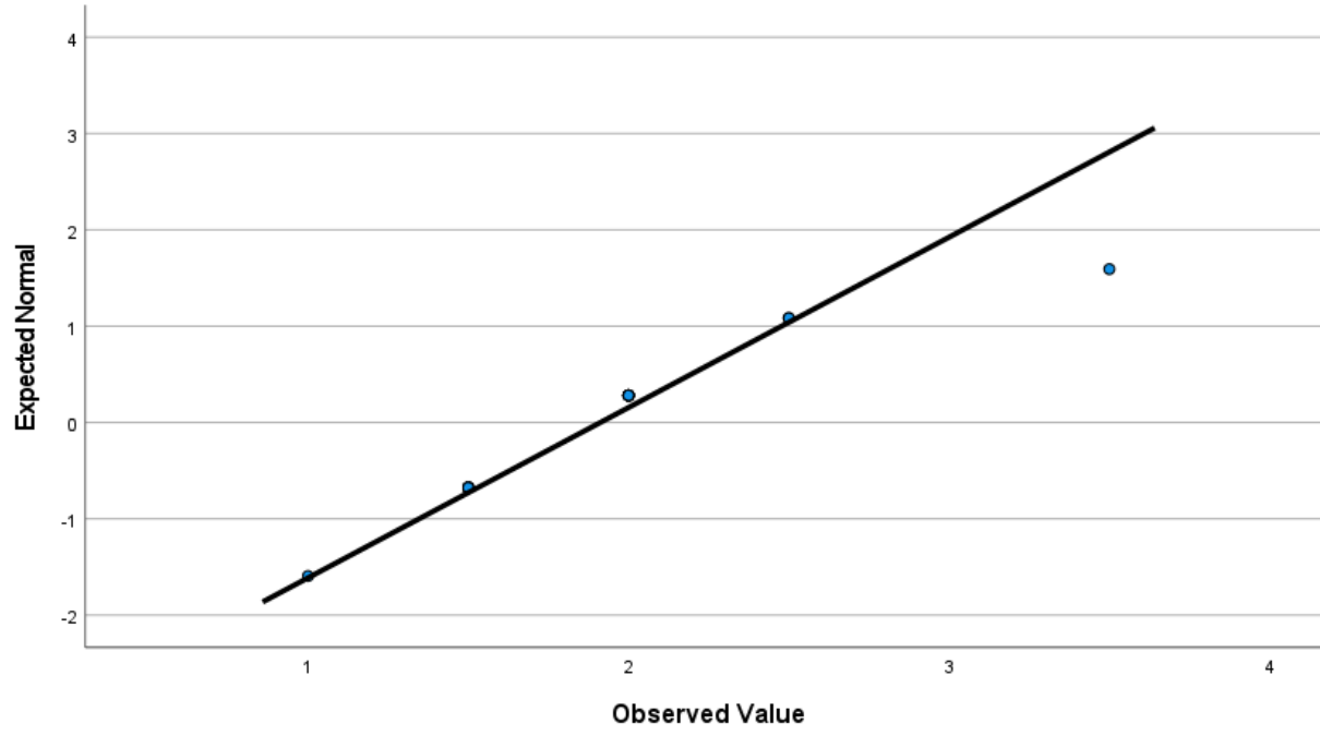
Normal Q-Q Plot of Post Overarching Concept
