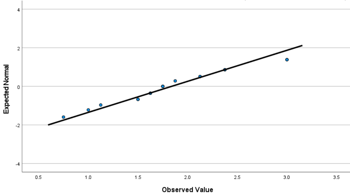
Normal Q-Q Plot of PreTPACKMean (Pre TPACK Overall Mean)
