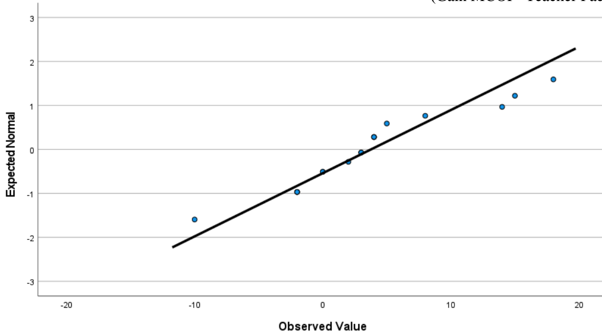
Normal Q-Q Plot of GainMCOP2Teacher (Gain MCOP 2 Teacher Facilitation)
