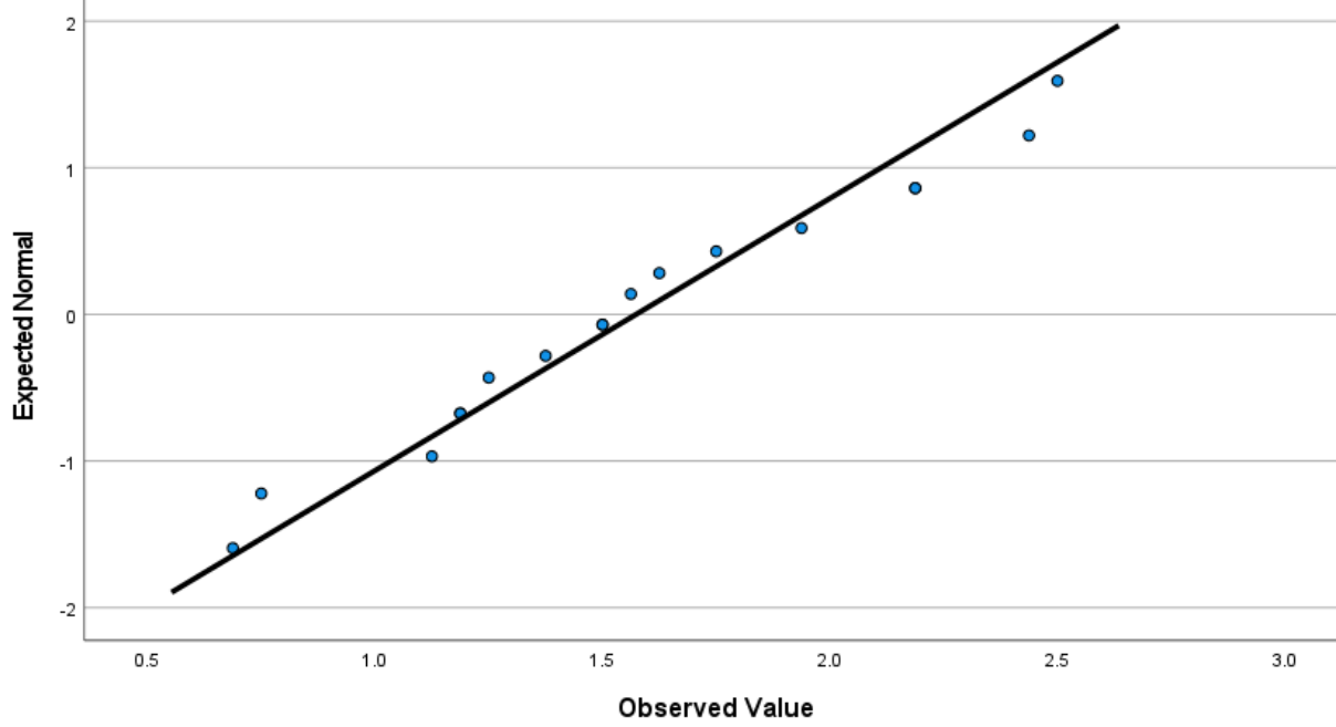
Normal Q-Q Plot of Post MCOP2 Total Mean
