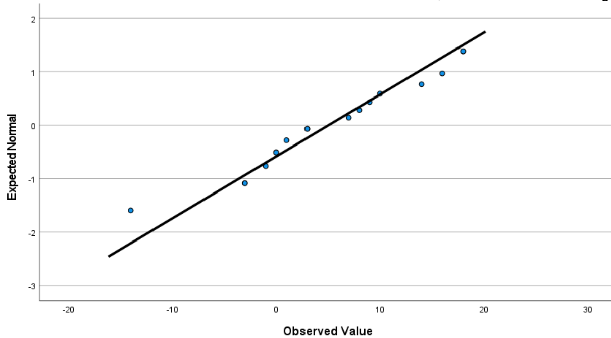
Normal Q-Q Plot of GainMCOP2Student (Gain MCOP 2 Student Engagement)
