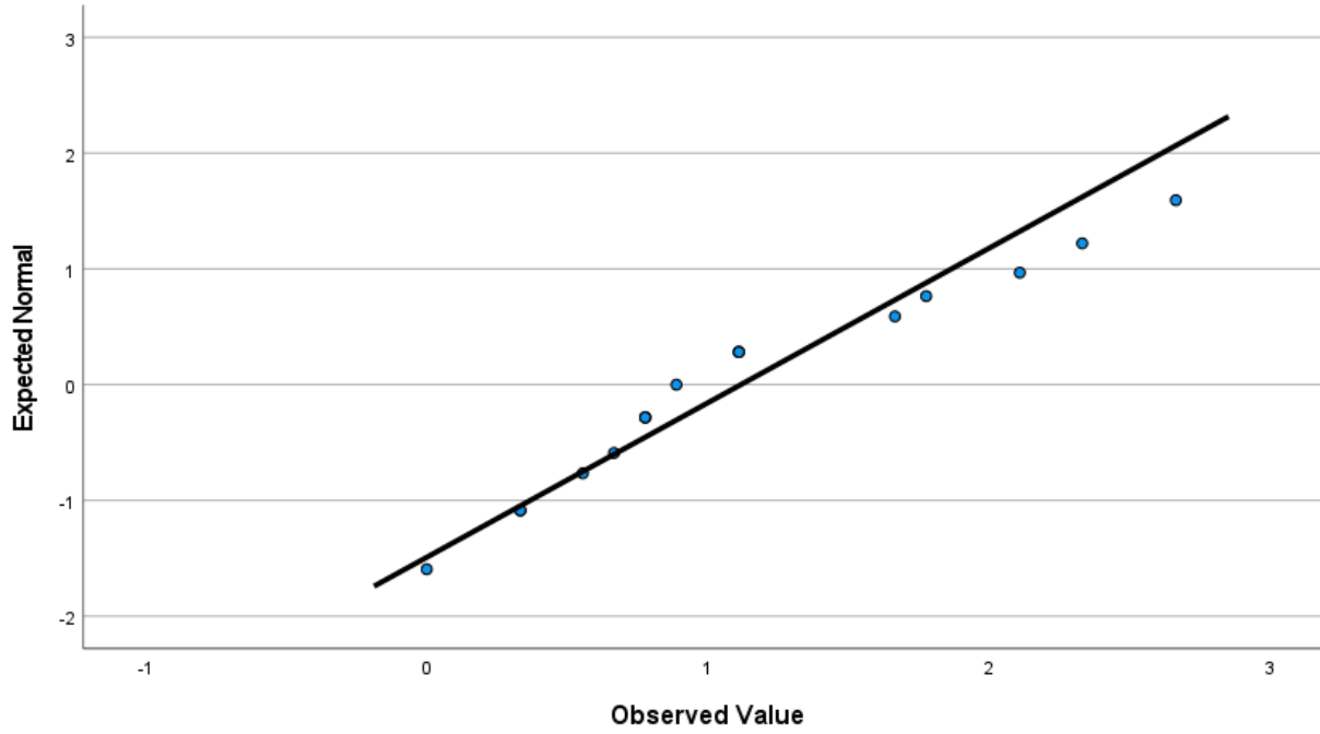
Normal Q-Q Plot of Pre MCOP2 Student Engagement Mean
