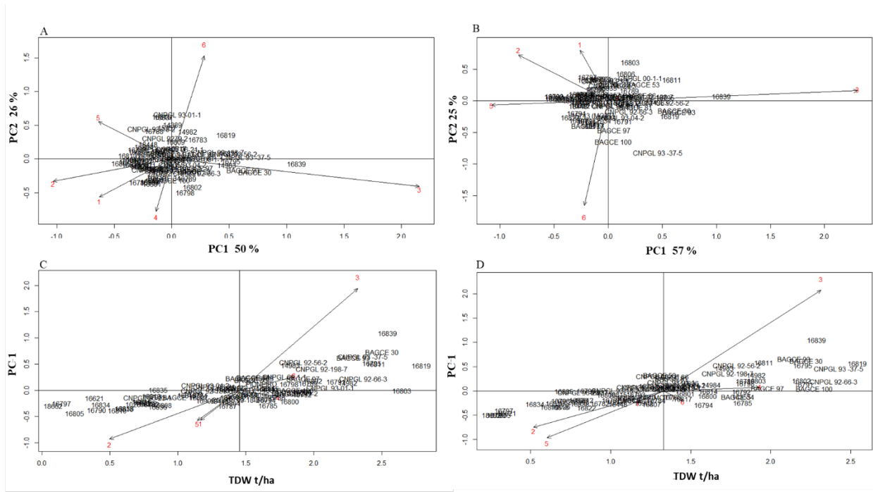
Figure 1. Biplots of an Additive Main effects and Multiplicative Interaction (AMMI) analysis of Principal component 1 (PC1) and Principal component 2 (PC2) upper lane A) Moderate water stress B) Severe water stress and biplot dry weight (TDW) vs PC1 lower lane C) moderate moisture stress and; D) severe moisture stress conditions with 84 Napier grass genotypes and 6 harvests (numbered in red) in the dry season.
