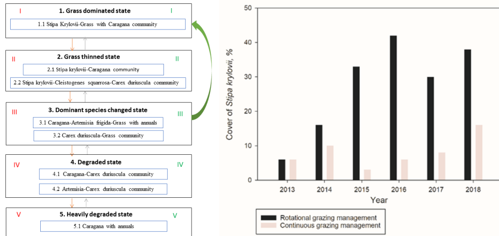
Figure 1. a) State and Transition model for Stipa krylovii -Grass with Caragana steppe rangeland; b) Perennial grass dynamics under contrasting management indicate the potential rate of recovery from State III to State I.
