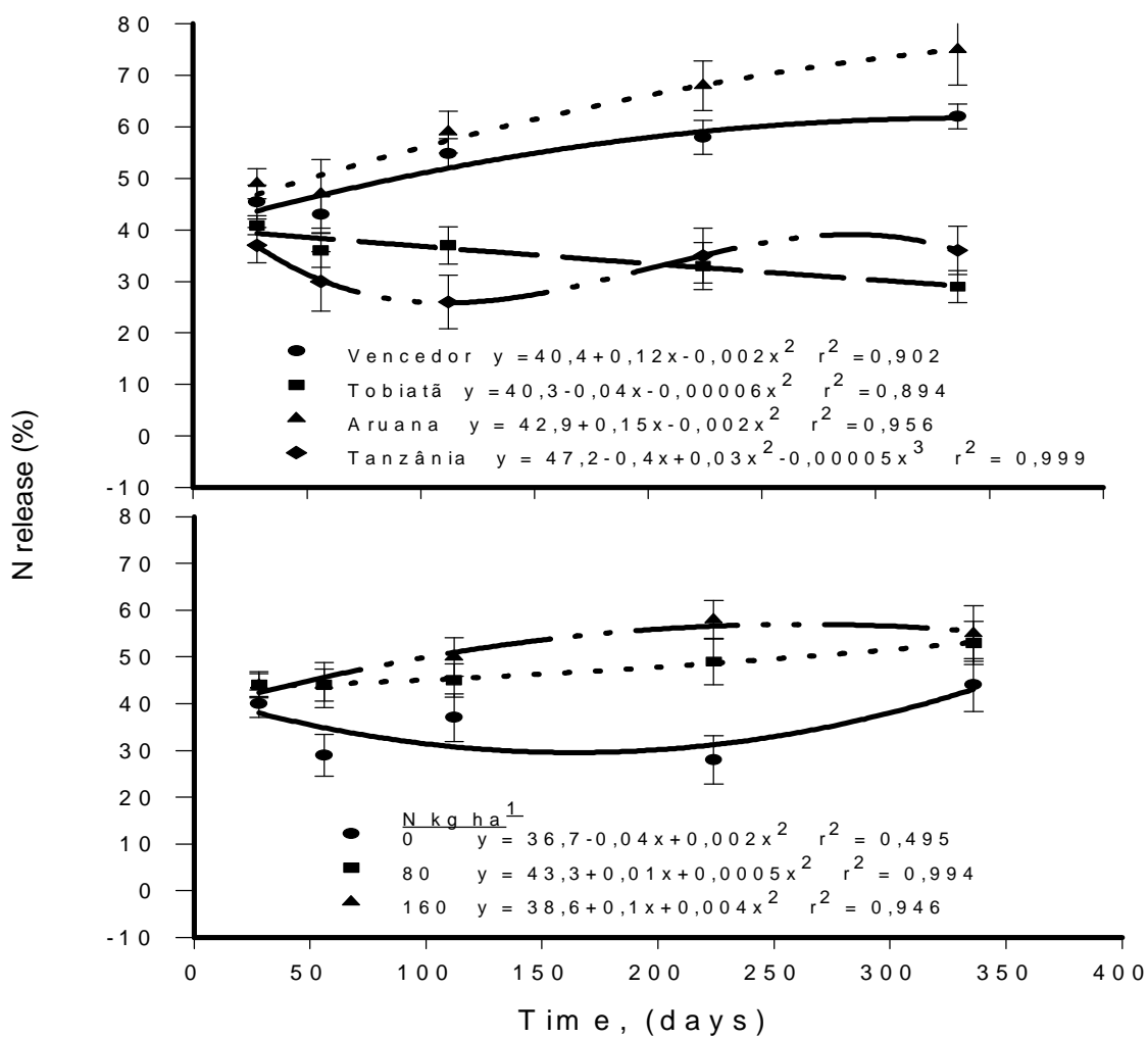
Figure 1 - Effect of cultivars and nitrogen fertilization on nitrogen release (%) from the litter of Panicum maximum in a Brazilian Alfisol
