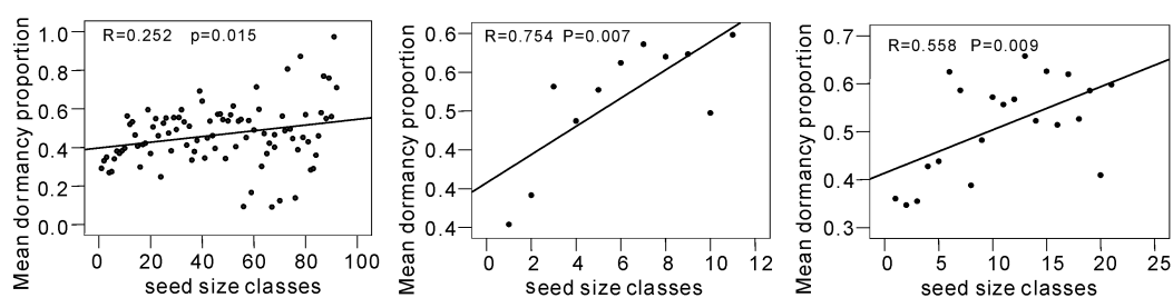
Figure 2 Simple linear regressions of mean proportion dormancy against seed mass
