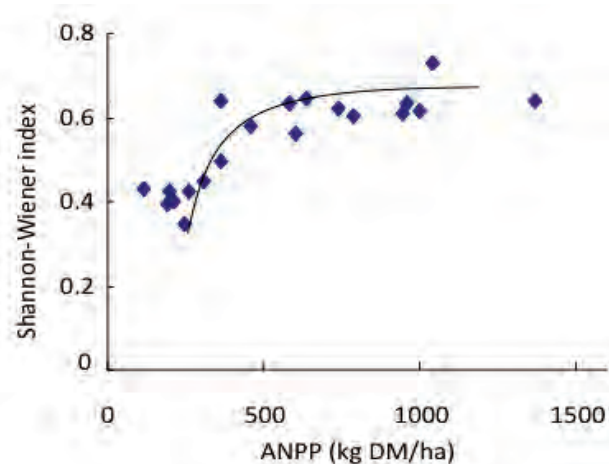
Figure 1. Annual net primary production (ANPP) and Shannon-Wiener diversity index for plant species under three stocking rates and for five summers on the desert steppe.
