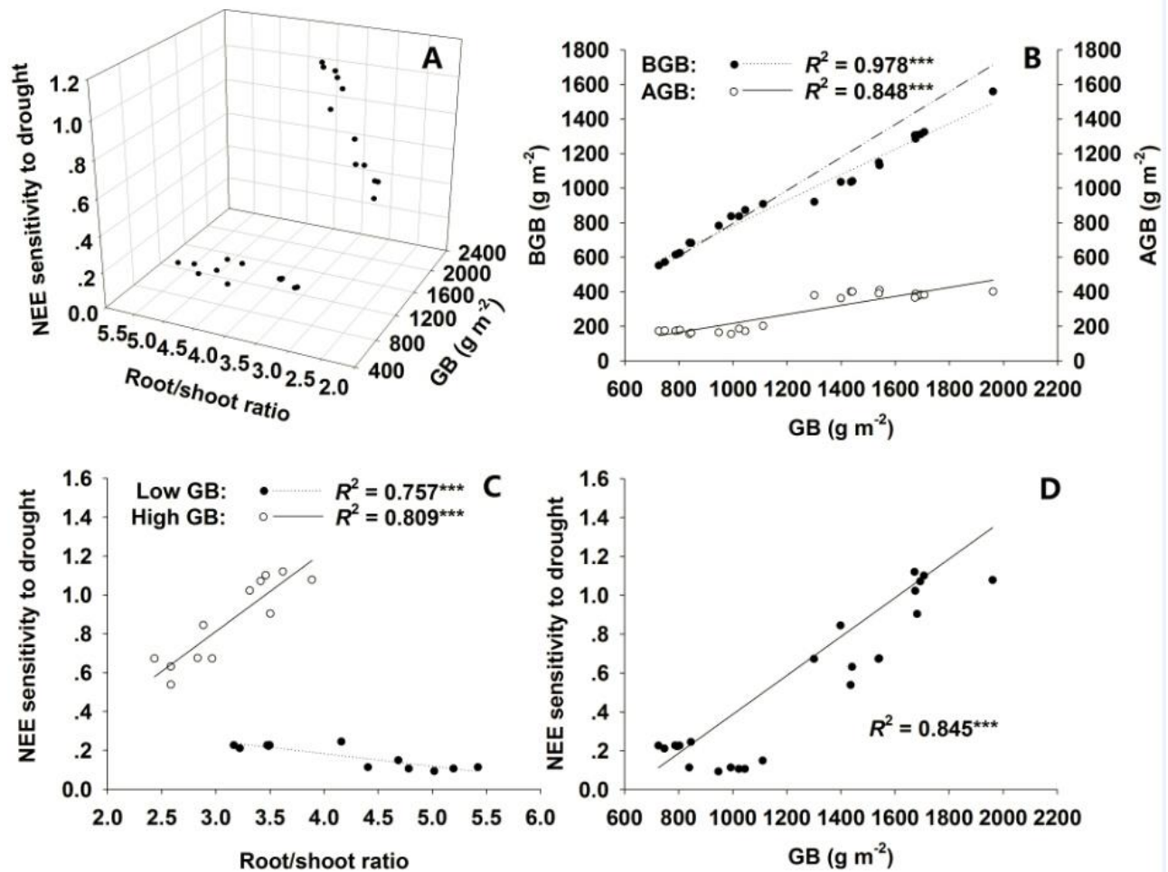
Fig. 2: Responses of the drought sensitivities of ecosystem carbon exchange ( S_{NEE} ) to (A) root/shoot ratio and gross biomass (GB, g\ m^{-2} ) in combination, (C) root/shoot ratio and (D) gross biomass (GB, g\ m^{-2} ). Dependence of aboveground biomass (AGB, g\ m^{-2} ) and belowground biomass (BGB, g\ m^{-2} ) on gross biomass (GB, g\ m^{-2} ) during the drought period (B). *** represents a significant correlation at the P < 0.001 level.
