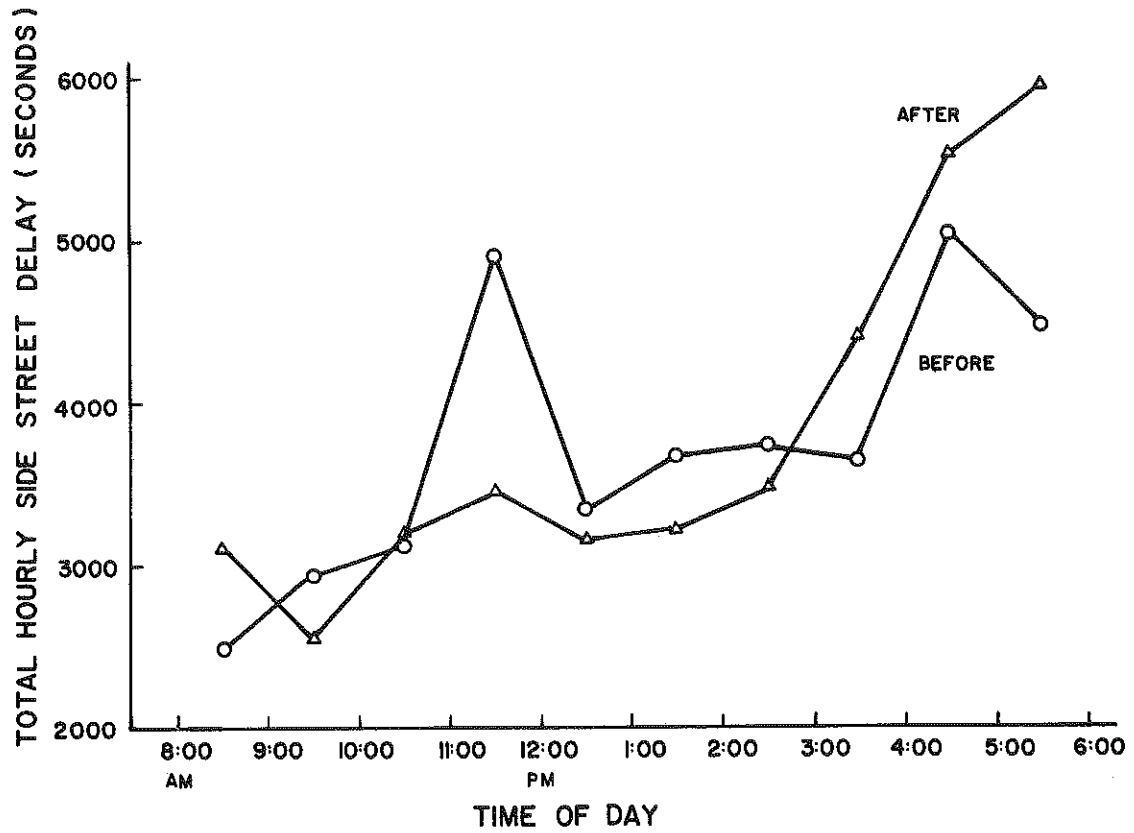
Figure 2. Side-Street Delay versus Time of Day at the Stanford Site before and after GES Installation.
