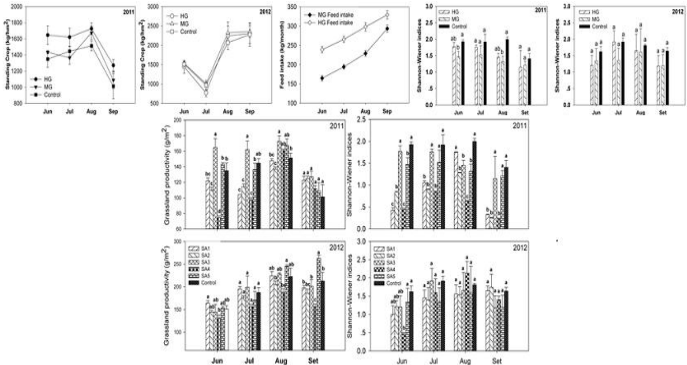
Fig. 1 Changes in plant biomass (standing crops), diversity index and animal intake with grazing intensities (2011-2012)
