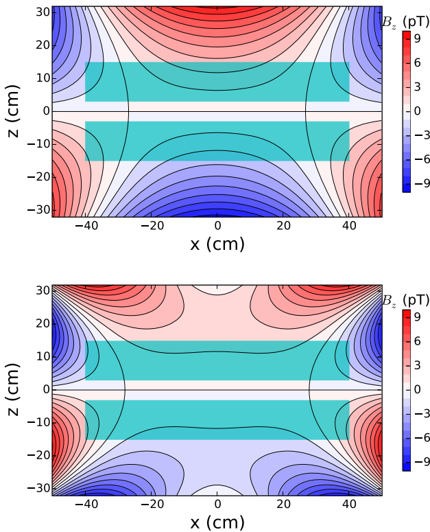
Fig. 10 Longitudinal component of the phantom modes. Top: phantom mode of order 3 B_z = \hat{G}_3 \hat{I}_{z,3} with \hat{G}_3 = 78 \text{ fT/cm} . Bottom: phantom mode of order 5 B_z = \hat{G}_5 \hat{I}_{z,5} with \hat{G}_5 = 78 \text{ fT/cm} . Both field configurations generate a false EDM of d_{n \leftarrow \text{Hg}}^{\text{false}} = 1 \times 10^{-27} \text{ e cm} . The light green rectangles represent the inner volume of the precession chambers
