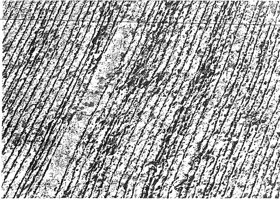
Figure 4. Some areas of the experimental PBC concrete bridge deck were deeply tyned, dislodging aggregates near the surface.
