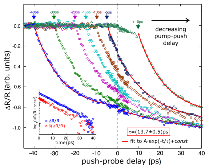
FIG. 2. Three pulse data with a weak push pulse insufficient to melt the magnetic order (see text) taken at T = 5 K. \Phi_{\text{push}} = 100 \mu\text{J}/\text{cm}^2 , \Phi_{\text{pump}} = 4 \mu\text{J}/\text{cm}^2 . The push pulse is at 0 ps; solid red lines: fits to a single exponential decay with the same time constant everywhere. Inset: logarithm of the signal before push pulse (blue) and the logarithm of the difference between the lowest (pump push delay \Delta t = -40 ps) and highest ( \Delta t = -5 ps) curves (red). As can be seen, a weak push pulse does not affect the relaxation dynamics.
