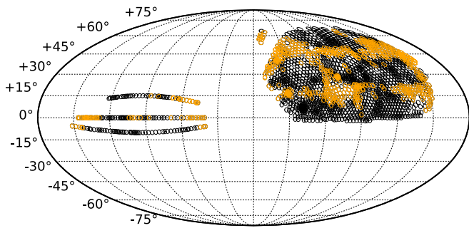
Figure 5. Planned MaNGA spectroscopic footprint in equatorial coordinates, centered at \alpha_{2000} = 270^\circ , with east to the left. Black shows the available MaNGA tiles; orange indicates example coverage for a simulated SDSS-IV MaNGA survey.
