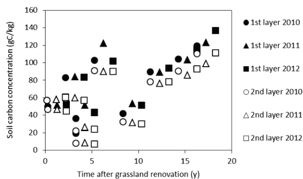
Figure 3. Relationship between the time after grassland renovation and soil carbon concentration in each layer. Treatment without manure application (0 Mg/ha/y) in all sites
