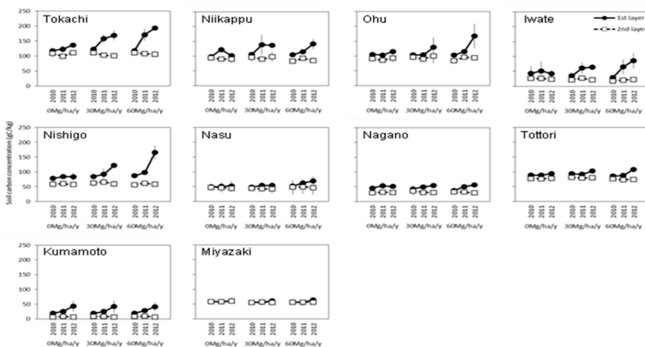
Figure 2. Inter-annual variations in soil carbon concentration of each treatment. Values represent means and standard deviations (n = 3)
