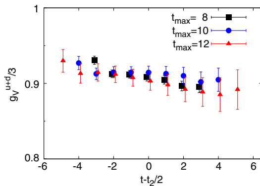
FIG. 5. The nucleon sink-source separation dependence of the matrix element with the vector charge for u + d in the connected insertion. Obviously, the larger t_2 , the worse the signal. The data points marked with the black squares ( t_2 = 8 ), the blue dots ( t_2 = 10 ) and the red triangles ( t_2 = 12 ) are consistent.
