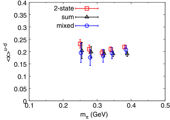
FIG. 13. The isovector quark momentum fraction ( \langle x \rangle^E in the rest frame) vs. the pion mass, from three fitting methods: 2-state fit (red squares), summed slope (black triangles), and the mixed fit which combines those two methods (blue dots). The results from the three methods are consistent.
