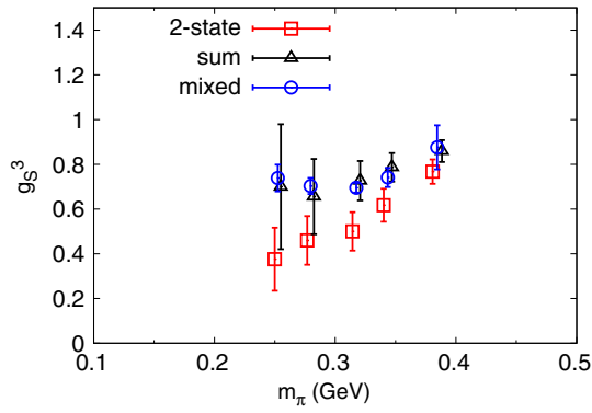
FIG. 10. Isovector scalar matrix element vs. pion mass from three kinds of fitting method: 2-state fit (red squares), summed slope (black triangles), and the mixed fit which combines those two methods (blue dots). The results from these different methods are slightly different.
