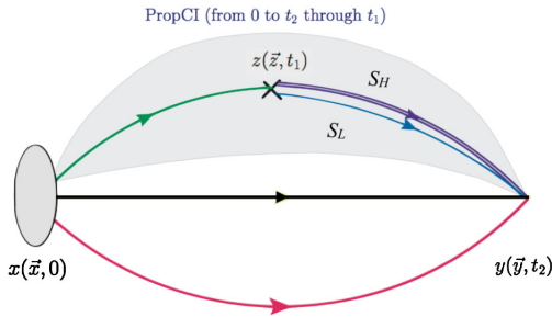
FIG. 2. The quark diagram of the proton correlation function with the connected insertion, from x to y , with an insertion at z . The product of the propagators in the shadowed region is the current inserted propagator, \hat{S} . The propagator from the current z to the sink y is decomposed into its low- and high-mode contributions ( S_L and S_H respectively) for further SNR/cost improvement from the advanced technique in the latter discussion. See Sec. III B for more details.
