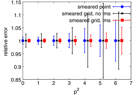
FIG. 1. The plot shows the relative error of 2pt as a function of the momentum squared p^2 at t = 8 in lattice units. The data points of the smeared grid cases have been shifted a bit on the abscissa to make it easier to distinguish them. The SNR of the case with the noise smeared grid source (red squares) and LMS applied is better than the one with smeared point source (blue dots), while the one with the noise smeared grid source but no LMS (black triangles) is even worse than the one with smeared point source.
