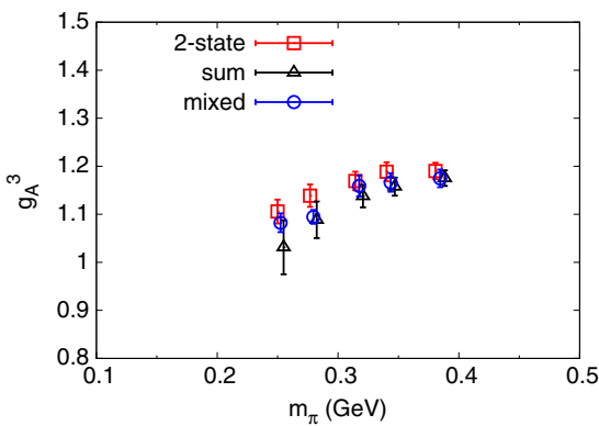
FIG. 8. The isovector axial-vector matrix element vs the pion mass, from three kinds of fitting method: 2-state fit (red squares), summed slope (black triangles), and the mixed fit which combines those two methods (the blue dots). The results from these different methods are consistent while that from the mixed method provides the best signal.
