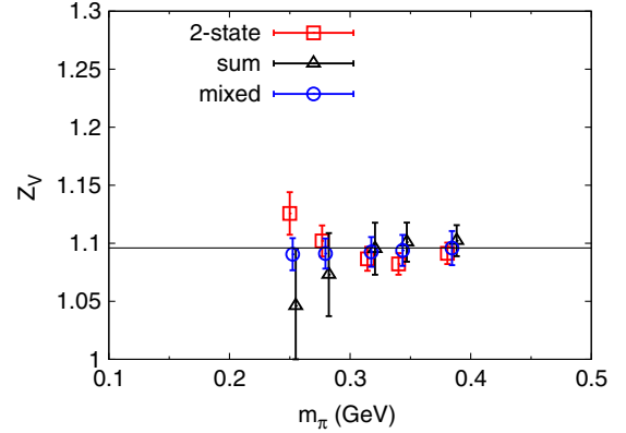
FIG. 6. The vector renormalization factor from the charge vs the pion mass, from three kinds of fitting methods: 2-state fit (red squares), summed slope (black triangles), and the mixed fit which combines those two methods (blue dots). The results from these different methods are consistent while that from the mixed method provides the best signal.
