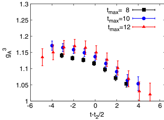
FIG. 7. The sink-source separation dependence of the matrix element of the isovector axial-vector current. The data of the isovector case with t_2 = 8 (black squares) are slightly smaller than that from the other two separations, while the result with t_2 = 10 (blue dots) is consistent with that with t_2 = 12 (red triangles).
