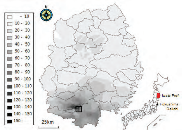
Figure 1. Soil radioactive material contents of Iwate Prefecture (Tsuiki and Maeda 2012a; 2012b, kBq/m 2 ). The square within the map is experimental area.
