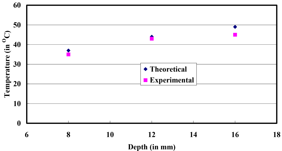
Figure 5.9: Comparisons for Drilling Depth
