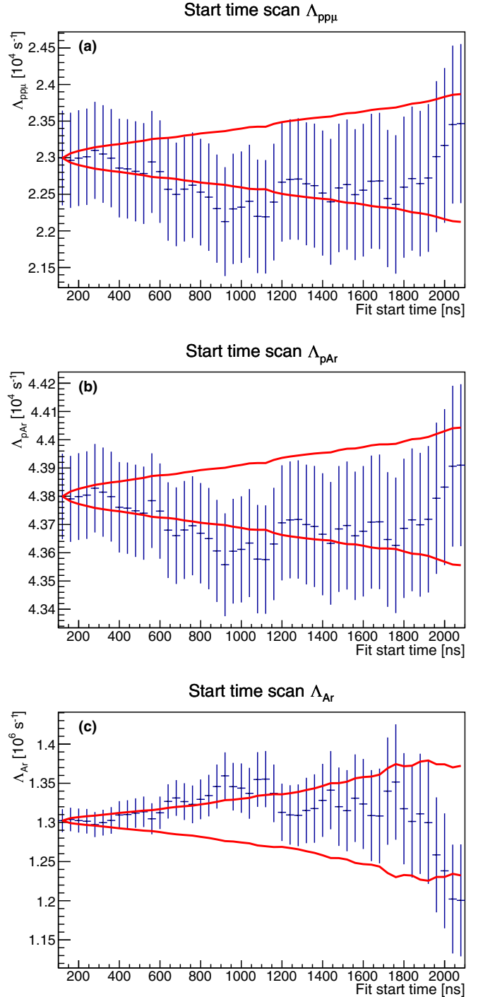
FIG. 6. (Color online) Fit results (blue points) versus fit start time for (a) \Lambda_{pp\mu} , (b) \Lambda_{pAr} , and (c) \Lambda_{Ar} . The variation of each rate is consistent with the expectations from the 1\sigma statistically allowed set-subset deviation (solid red line).
