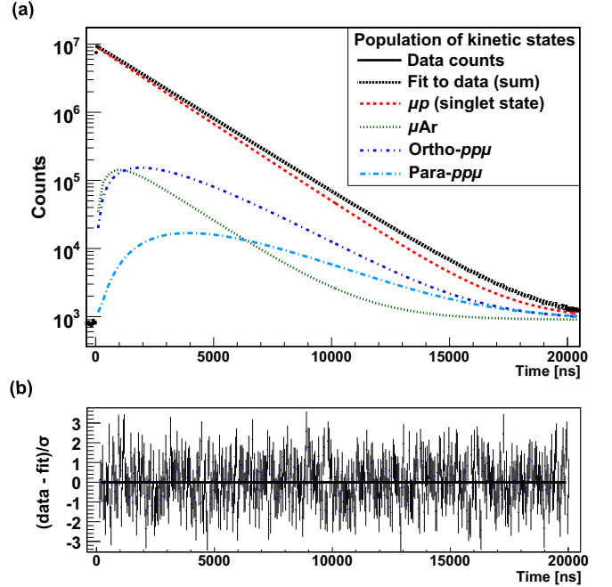
FIG. 5. (Color online) (a) Fit to the decay electron time spectrum using Eq. (13). The data are shown as the black line. The colored curves depict the time-dependent contributions from the kinetic states; the black dashed line is the fitted sum. (b) The normalized residuals between the data and the fit function, (N_i - N(t_i))/\sigma_i , indicate good agreement in the fitted range 0.12–20 \mu s.
