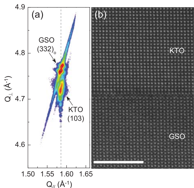
FIG 4. X-ray RSM and STEM data. (a) X-ray RSM around the GSO (332) o plane. The vertical dashed line indicates that the KTO film is fully strained to the GSO substrate. (b) HAADF cross-sectional STEM image of the KTO/GSO heterointerface. The white line is a 5 nm scale bar. The heterointerface between KTO and GSO is marked by a triangle (◄).
