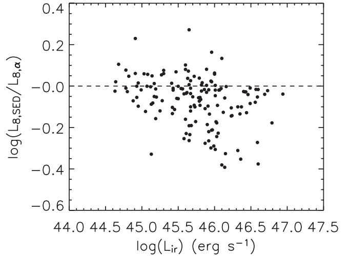
FIG. 6.—Logarithmic ratio of L_{8,SED} ( L_{8 \mu\text{m}} determined from the R06a mean composite SED normalized to photometry within 0.3 dex of rest-frame 8 \mu\text{m} ) to L_{8,\alpha} ( L_{8 \mu\text{m}} calculated by extrapolating to 8 \mu\text{m} from the mid-infrared power-law model) vs. \log(L_{IR}) . For reference, a horizontal dashed line marks a ratio of unity. The strong decrease in L_{8,SED}/L_{8,\alpha} with increasing L_{IR} indicates increasing spectral curvature at higher luminosities.
