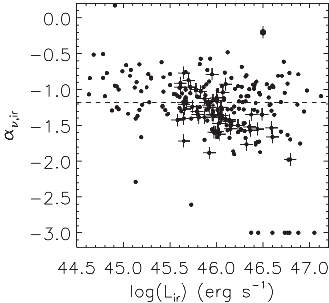
FIG. 5.—Infrared spectral index, \alpha_{\nu,IR} , vs. \log(L_{IR}) for the SED sample (filled circles); the subset of the SED sample with z = 1.0 – 1.5 is also marked with plus signs. The parameter \alpha_{\nu,IR} is determined from power-law fits ( l_{\nu} \propto \nu^{\alpha_{\nu,IR}} ) to the Spitzer photometry between rest-frame 1.8 and 8.0 \mu\text{m} ; the eight quasars at z > 3.5 (plotted at \alpha_{\nu,IR} = -3.0 ) only had one photometric data point in the bandpass; they are not included in the analysis. For reference, a horizontal dashed line marks the median \alpha_{\nu,IR} value; for higher values of L_{IR} a larger fraction of quasars lie below the median. The median uncertainty in \alpha_{\nu,IR} from fitting a power-law model to the photometry is indicated as a vertical error bar on a large, filled circle in the upper right corner of the plot.
