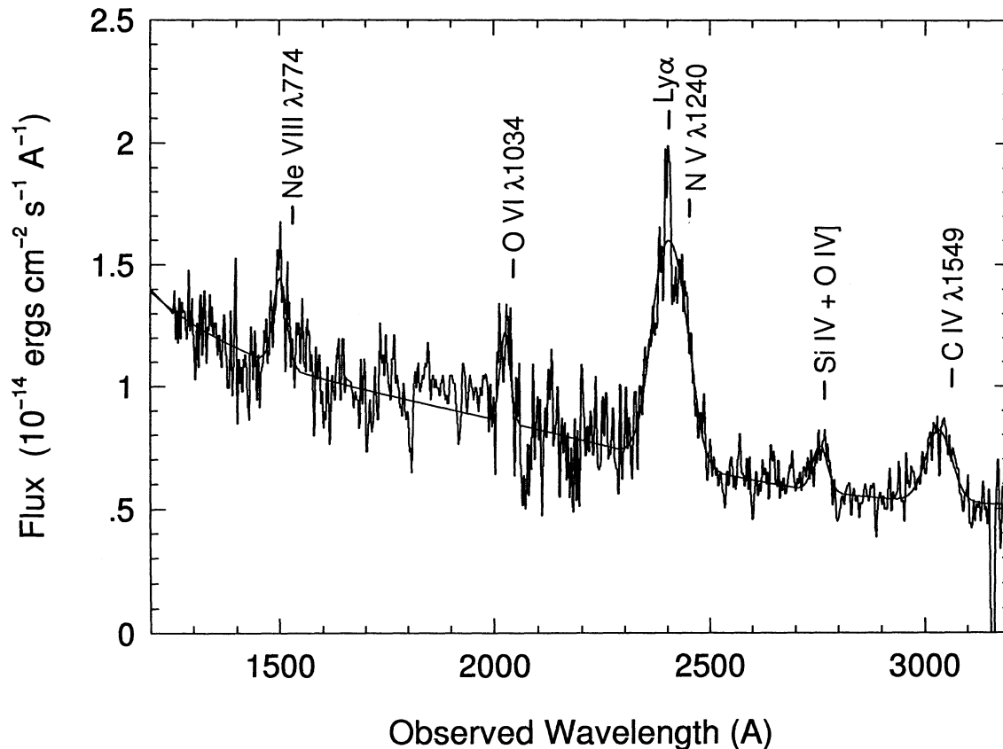
FIG. 1.—Co-added IUE spectra of PG 1148+549 plotted at the observed wavelengths. The short- and long-wavelength data join without overlap at \sim 1970 Å, which causes a slight discontinuity in the plotted continuum. The spectra are smoothed with a 3 pixel-wide boxcar function. The prominent emission lines are labeled at the published redshift of z_e = 0.978 . The smooth, solid line is a polynomial fit to the continuum, with single Gaussian fits to each of the labeled lines. The Ne VIII and C IV velocity widths are similar despite their different appearances in this figure.
