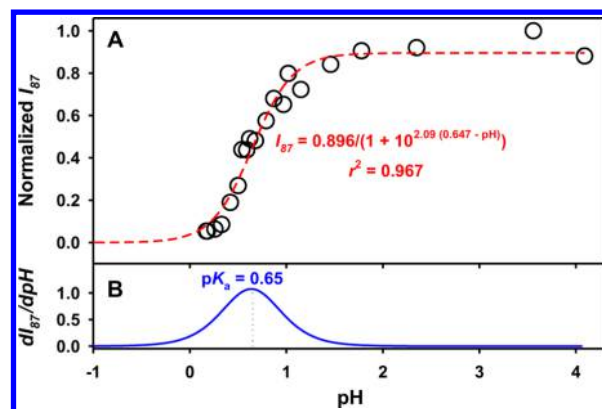
Figure 5. (A) OESI-MS titration curve for pyruvic acid (from a solution in water) deposited on the surface of water for microdroplets exposed to 1.40 ppmv ( \cong 3.28 \times 10^{13} molecules \text{cm}^{-3} ) under the experimental conditions for a contact time \tau_c = 1 \mu\text{s} . (O) Normalized ion count for the acetate anion at m/z 87, I_{87} , as a function of pH fitted with a (red line) sigmoid curve with the coefficient of correlation r^2 = 0.967 . (B) First derivative of the sigmoid curve in (A), where the maximum corresponds to the pK_a (blue line).
