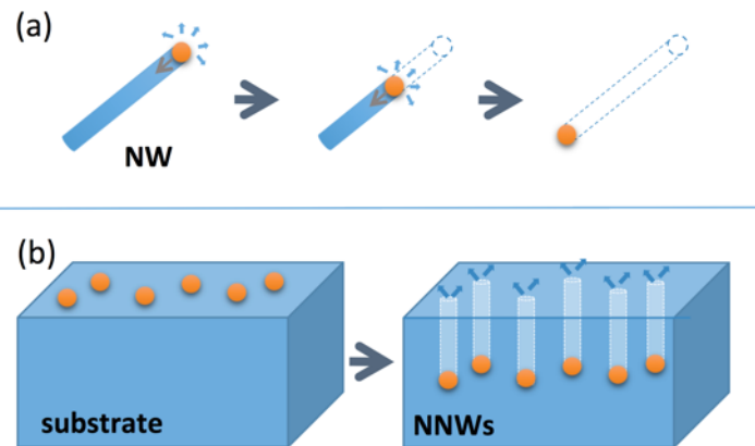
Figure 1.4 Cartoon showing (a) SLV dissolution of a single NW and (b) SLV formation of negative NWs.
