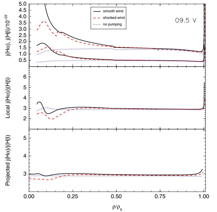
Figure 13. As in Figure 10, for the case of an O9.5 V star. (A color version of this figure is available in the online journal.)
