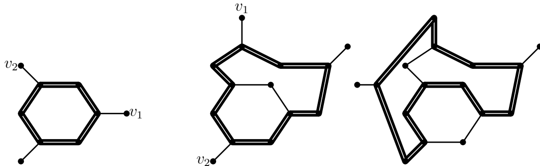
Figure 3.9: On the left most picture we start with a clawed cycle. Choosing two points, v_1 and v_2 we attach a clawed path of length 2. Since the chosen two leaf claws are incident, we pair the toggle edges of each. Then we choose two more vertices, v_1 and v_2 and continue. In this step there is one claw unit that is incident to two leaf claws and the other claw unit is incident to one.
