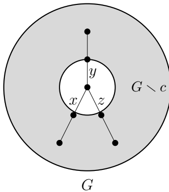
Figure 3.2: The edge set \{x, y, z\} defines an induced claw unit, call it c , of graph G . The shaded region is the graph G \setminus c .
