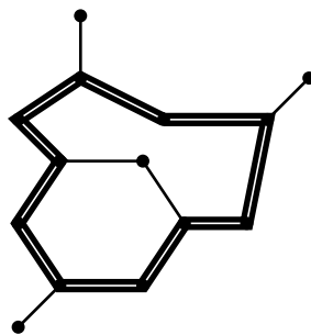
Figure 3.7: Clawed non-separable graph which attains the maximum attaching sites.
