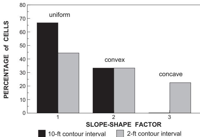
Figure 7. Impact of contour resolution on AGNPS slope-shape factor for catchment B.
