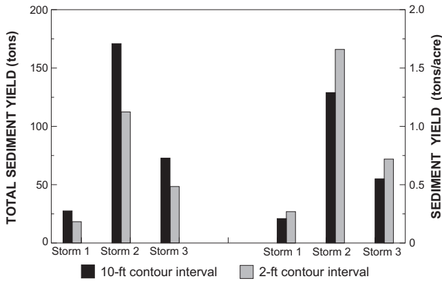
Figure 15. Sediment yields predicted by AGNPS for storms 1, 2, and 3 in catchment A.
