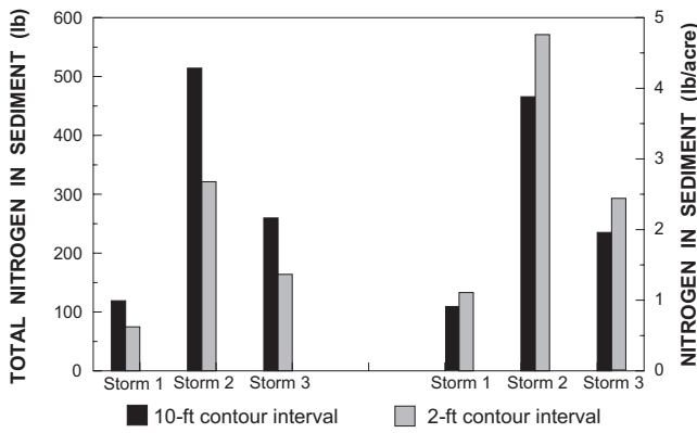
Figure 20. Sediment-borne nitrogen load predicted by AGNPS for storms 1, 2, and 3 in catchment A.
