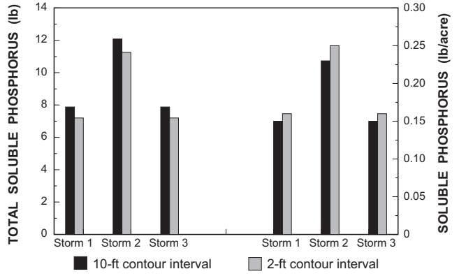
Figure 23. Soluble phosphorus load predicted by AGNPS for storms 1, 2, and 3 in catchment B.
