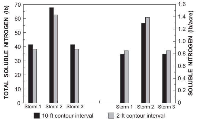
Figure 19. Soluble nitrogen load predicted by AGNPS for storms 1, 2, and 3 in catchment B.
