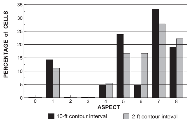
Figure 4. Impact of contour resolution on AGNPS cell aspect for catchment B.
