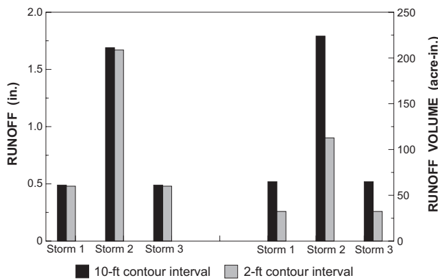
Figure 12. Surface runoff predicted by AGNPS for storms 1, 2, and 3 in catchment A.
