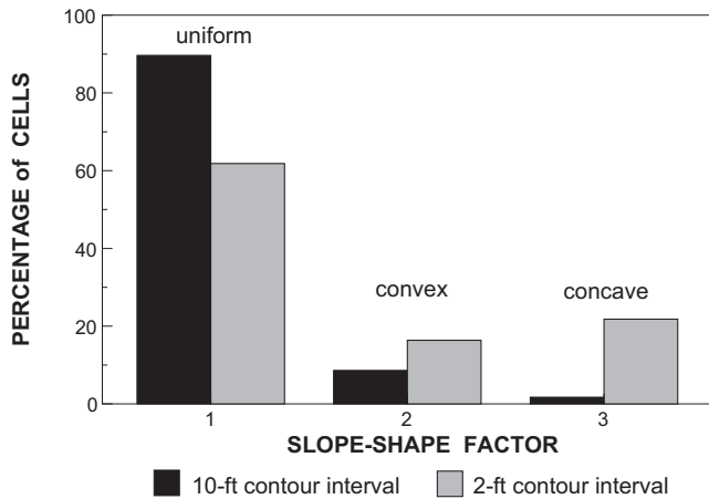
Figure 6. Impact of contour resolution on AGNPS slope-shape factor for catchment A.
