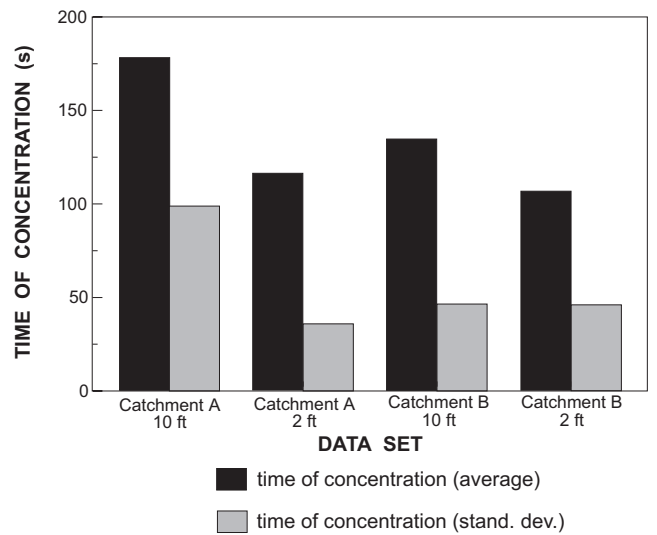
Figure 11. Impact of contour resolution on time of concentration.
