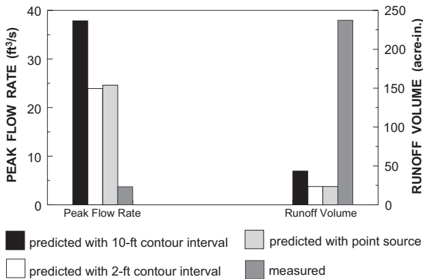
Figure 31. Predicted and measured peak flow rates and runoff volumes for storm 5 in catchment A*.
