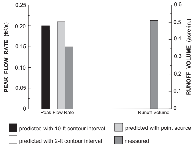
Figure 32. Predicted and measured peak flow rates and runoff volumes for storm 6 in catchment A*.
