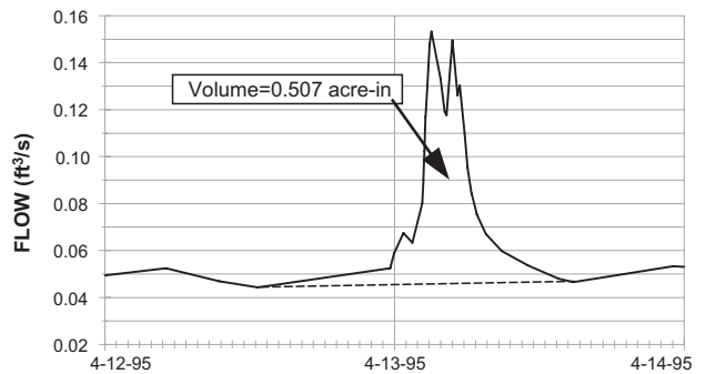
Figure 28. Observed runoff for storm 6 in catchment A*. Catchment A* resulted from approximately 35 acres being added to catchment A to accommodate the location of a weir installed to collect flow data.
