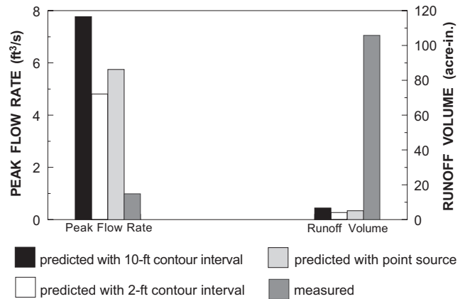
Figure 30. Predicted and measured peak flow rates and runoff volumes for storm 4 in catchment A*. Catchment A* resulted from approximately 35 acres being added to catchment A to accommodate the location of a weir installed to collect flow data.
