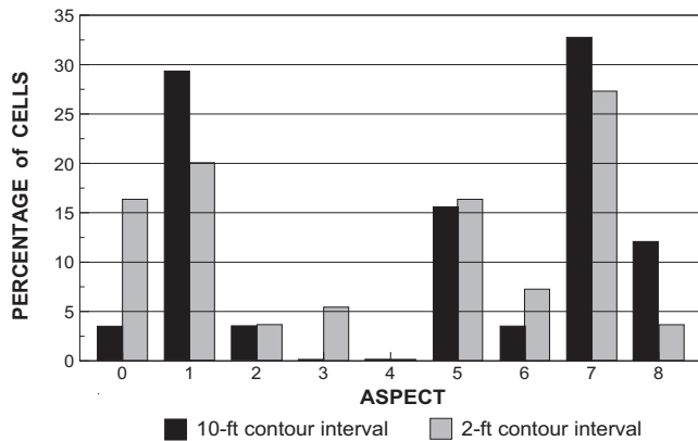
Figure 3. Impact of contour resolution on AGNPS cell aspect for catchment A.
