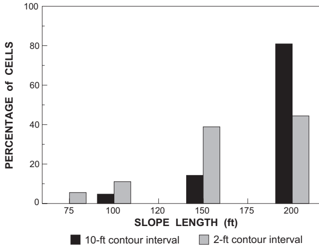
Figure 9. Impact of contour resolution on slope length for catchment B.
