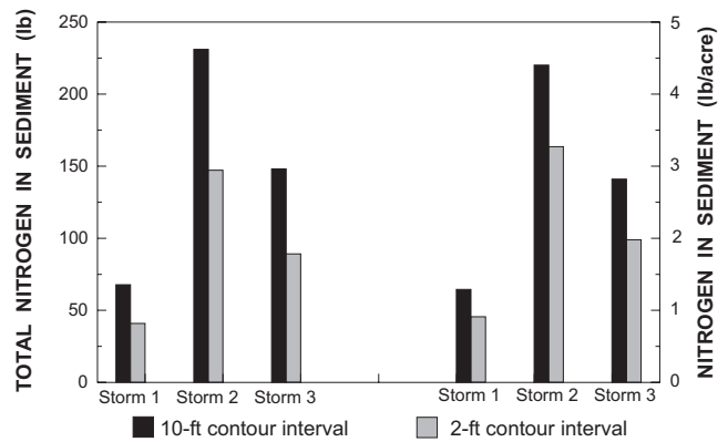
Figure 21. Sediment-borne nitrogen load predicted by AGNPS for storms 1, 2, and 3 in catchment B.
