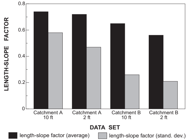
Figure 10. Impact of contour resolution on USLE length-slope factor.
