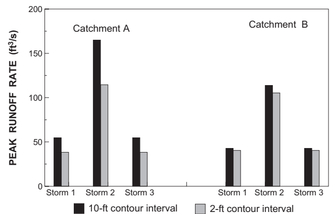
Figure 14. Peak runoff rates predicted by AGNPS for storms 1, 2, and 3.
