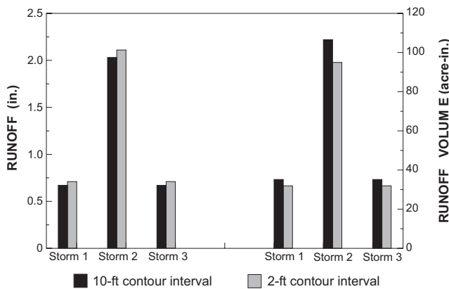
Figure 13. Surface runoff predicted by AGNPS for storms 1, 2, and 3 in catchment B.
