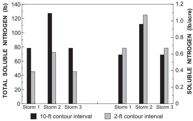
Figure 18. Soluble nitrogen load predicted by AGNPS for storms 1, 2, and 3 in catchment A.
