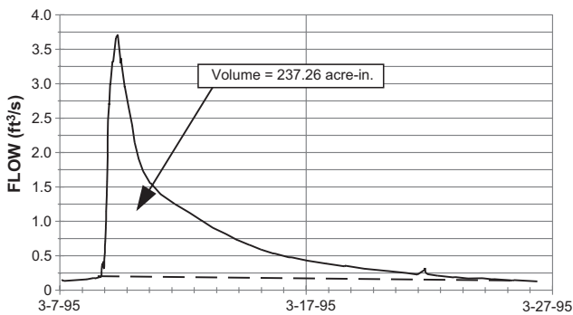
Figure 27. Observed runoff for storm 5 in catchment A*. Catchment A* resulted from approximately 35 acres being added to catchment A to accommodate the location of a weir installed to collect flow data.
