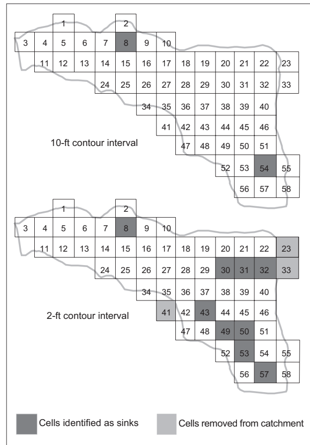
Figure 5. Cells identified as sinks, and cells removed from catchment, using 10-ft (top) and 2-ft (bottom) contour intervals.
