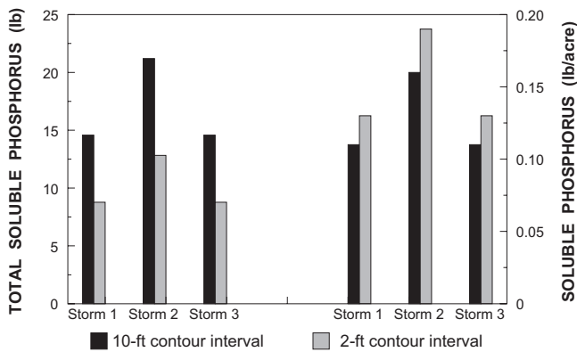
Figure 22. Soluble phosphorus load predicted by AGNPS for storms 1, 2, and 3 in catchment A.
