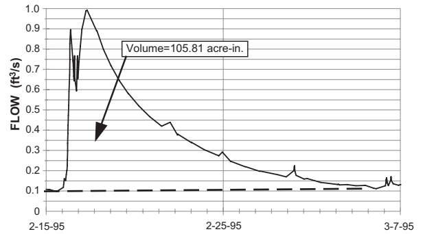
Figure 26. Observed runoff for storm 4 in catchment A*. Catchment A* resulted from approximately 35 acres being added to catchment A to accommodate the location of a weir installed to collect flow data.
