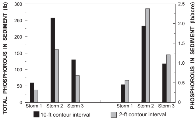
Figure 24. Sediment-borne phosphorus load predicted by AGNPS for storms 1, 2, and 3 in catchment A.
