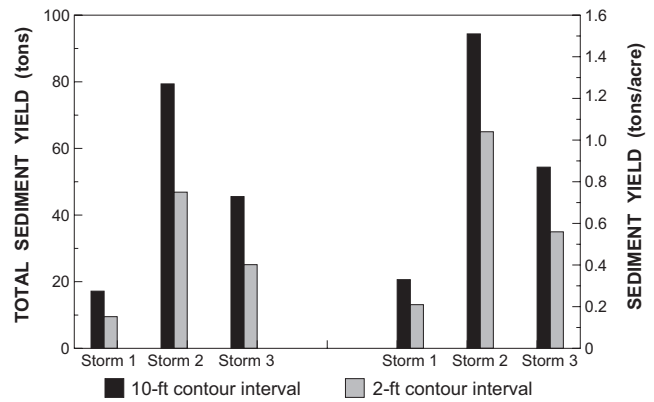
Figure 16. Sediment yields predicted by AGNPS for storms 1, 2, and 3 in catchment B.
