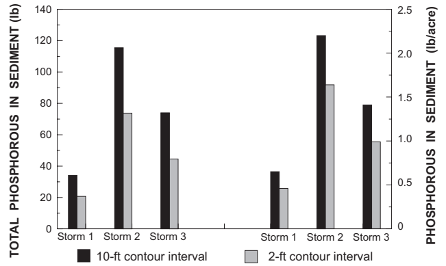
Figure 25. Sediment-borne phosphorus load predicted by AGNPS for storms 1, 2, and 3 in catchment B.
