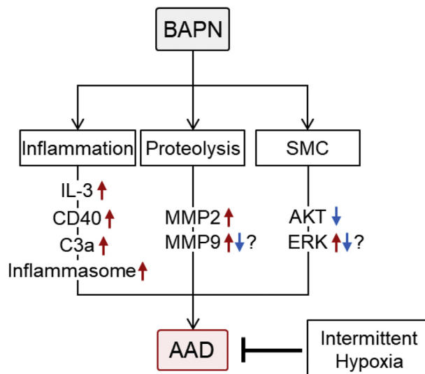
Fig 1. Molecular mechanisms studied in \beta -aminopropionitrile (BAPN)-induced aortic aneurysm and dissection (AAD) mouse model. IL , Interleukin; MMP , metalloproteinase; SMC , smooth muscle cell.
