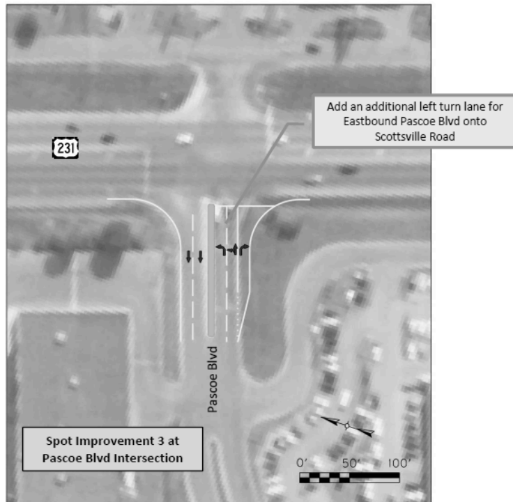
Figure 54: Pascoe Blvd Improvements
