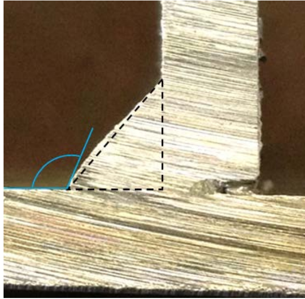
Fig. 4.6 A Cross Section of Weld Bead in “Small-Root opening” Experiment
