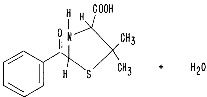
THIAZOLIDINE-DERIVATIVE OF PHENYLGLYOXAL
