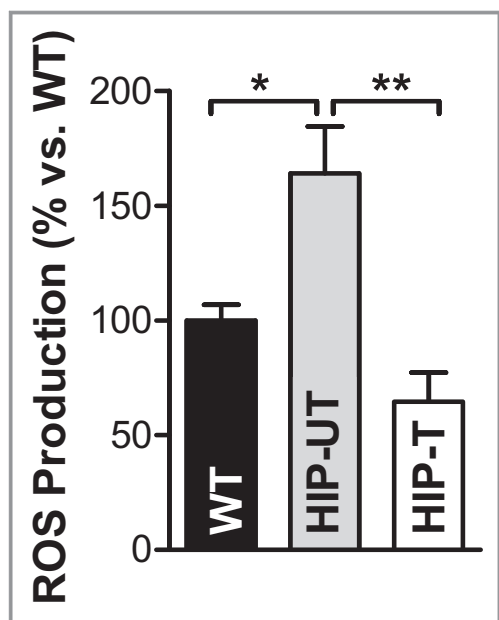
Figure 7. APAU treatment reduces amylin oligomer-induced oxidative stress. ROS production measured with CM-H 2 DCFA in myocytes from WT (8 myocytes from 4 rats), untreated HIP (HIP-UT; 13 cells, 4 rats), and treated HIP (HIP-T; 9 cells, 3 rats) rats. * P <0.05, ** P <0.01. APAU indicates (1-(1-acetypiperidin-4-yl)-3-adamantanyure; CM-H 2 DCFA, 5-(and-6)-chloromethyl-20,70-dichlorodihydrofluorescein diacetate acetyl ester; ROS, reactive oxygen species; WT, wild-type.
