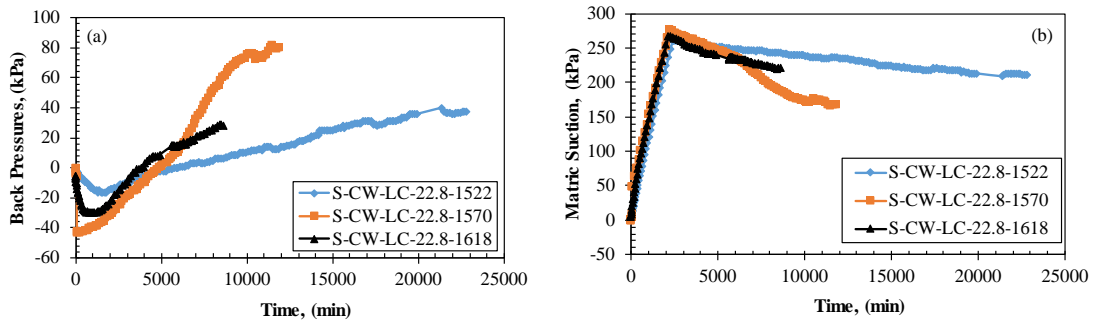
Figure H.15 Equilibrium phase CW triaxial tests experimental data for the LCesilt at different initial densities
