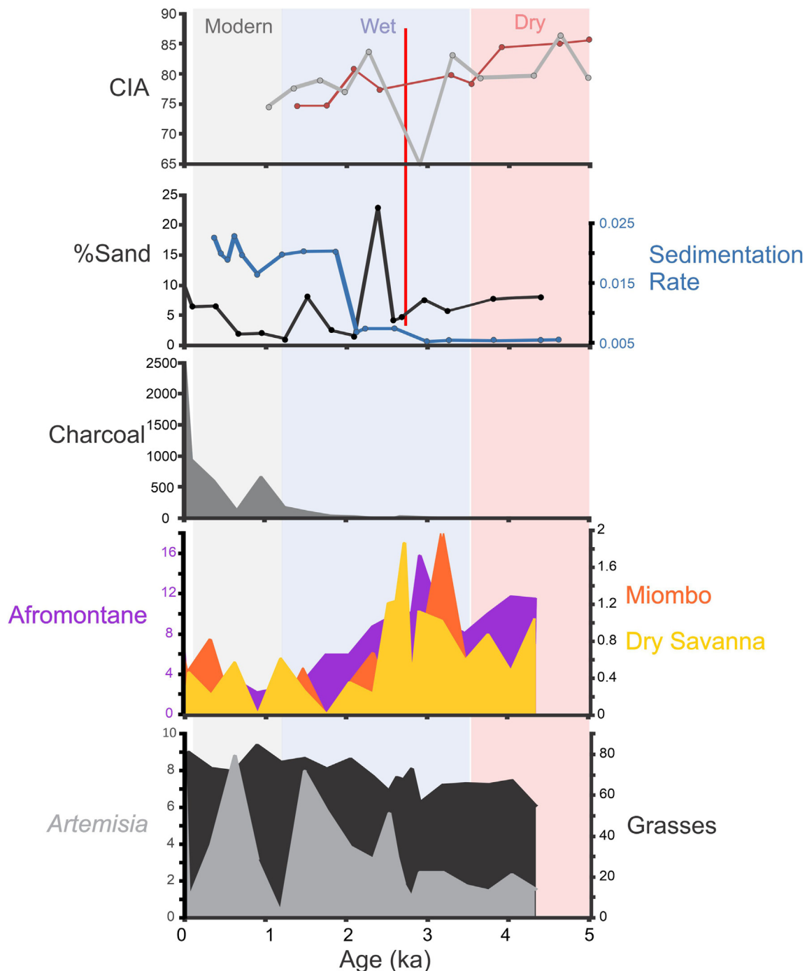
Fig. 3. Late Holocene sedimentological and palynological indicators from core LT-98-2M from off of the Mahale Mountains as well as the chemical index of alteration (CIA) calculated on KH3. For CIA, the red line is a 5 point running mean of the original dataset. All pollen data is reported in relative abundances (%). Charcoal influxes are in units of pieces/cm 2 /yr. Sedimentation rates are in m/yr. Red rectangle indicates dry climate, blue rectangle indicates wet climate, grey indicates near modern climate. Red line denotes the position of a significant change point with respect to mean and variability for grain size and CIA data, where the red line crosses a timeseries it represents a significant change in that series.
