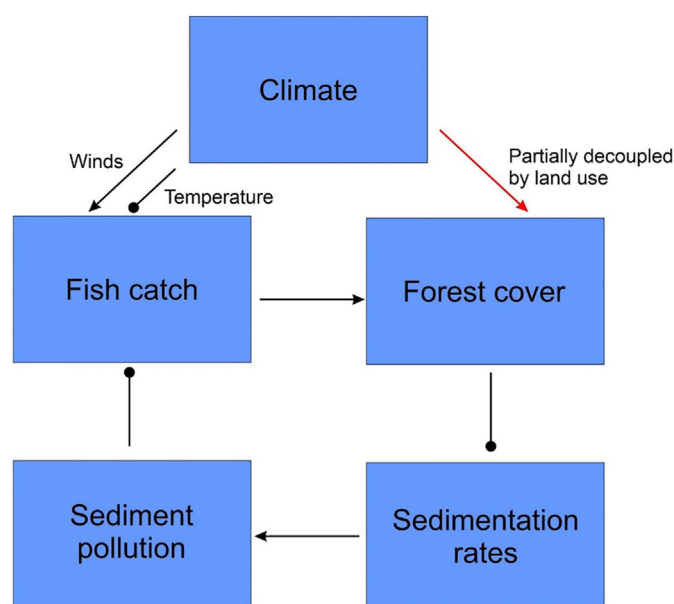
Fig. 6. Systems diagram showing the linkage between climate, fish catch, and deforestation. Arrows represent positive couplings and lines with circles represent negative coupling. The red arrow linking climate and forest cover denotes that this natural coupling is partially decoupled by land use based on sediment core data.
