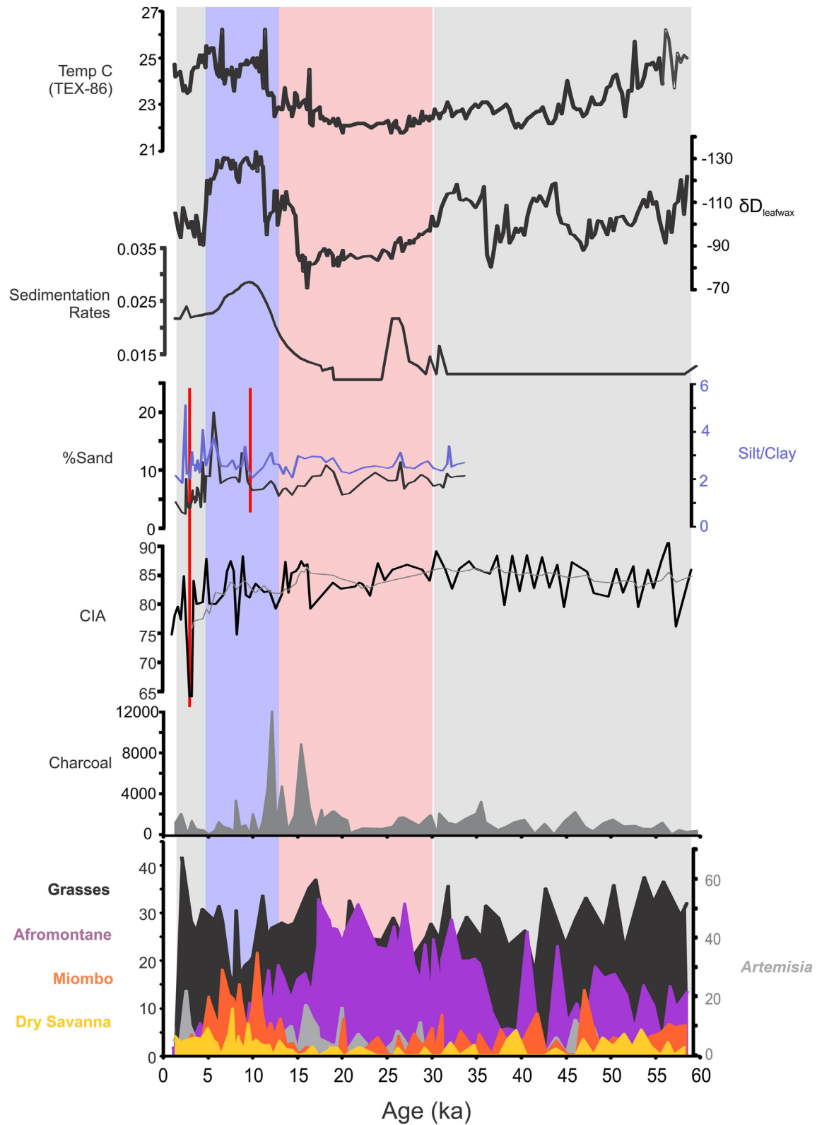
Fig. 2. Late Pleistocene-Holocene climate (TEX-86 and \delta D_{wax} ; Tierney et al., 2008; 2010), sedimentological (chemical index of alteration [CIA], sedimentation rates, terrigenous grain size), and palynological (pollen and charcoal) indicators from cores KH3 and KH4 from Kalya Horst and Platform. For CIA, the light grey line is a 5 point running mean of the original dataset. All pollen data is reported in relative abundances (%). Charcoal influxes are in units of pieces/cm 2 /yr. Sedimentation rates are in m/yr. The red rectangle means drier than modern conditions, the blue rectangle means wetter than modern conditions, and grey means circa-modern conditions. Red line denotes the position of a significant change point with respect to mean and variability for grain size and CIA data, where the red line crosses a timeseries it represents a significant change in that series.
