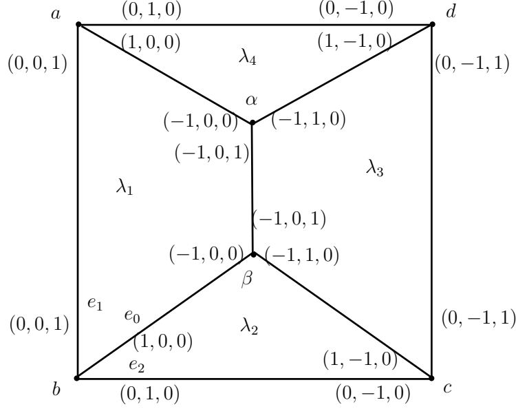
Figure 3.4: (\mathbb{C}P^2 \# \mathbb{C}P^2)^w with Edge, Basis and Facet Vectors
