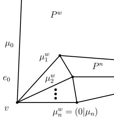
Figure 3.5: Edge Vectors of the Canonical Wedge
