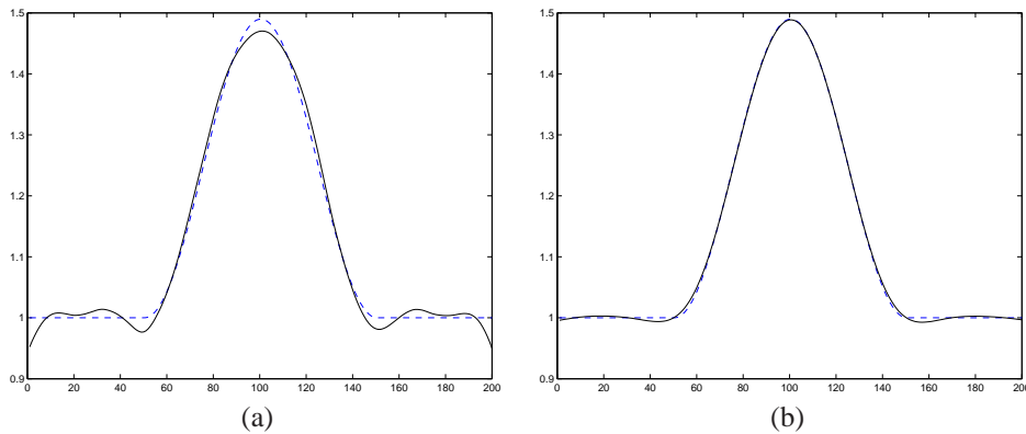
FIGURE 4.2. Example 4.2: Approximate solutions \mathbf{x}_{k,\mu} computed by the Arnoldi-Tikhonov method with the regularization parameter \mu determined by the discrepancy principle. The dashed curves show the vector \hat{\mathbf{x}} ; the continuous curves display in (a) the approximate solution \mathbf{x}_{10,\mu} determined with regularization operator L := I and in (b) the approximate solution \mathbf{x}_{7,\mu} determined with L := L_{1,0} .
