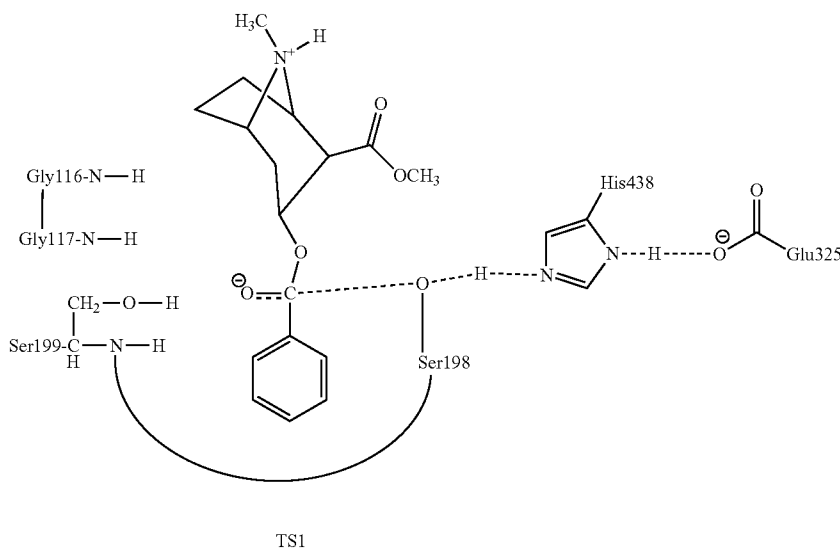
Scheme 5. Schematic representation of the transition-state structure for first reaction step for (-)-cocaine hydrolysis catalyzed by a BChE mutant with an A199S mutation.
