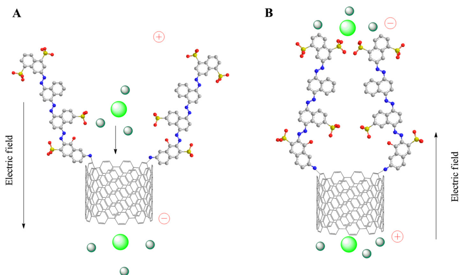
Figure 4 Schematic mechanism of ionic rectification on DWCNT-dye membrane (A, B). Gray, C; blue, N; red, O; yellow, S; light green, \text{Fe}(\text{CN})_6^{3-} ; dark green, \text{K}^+ .
