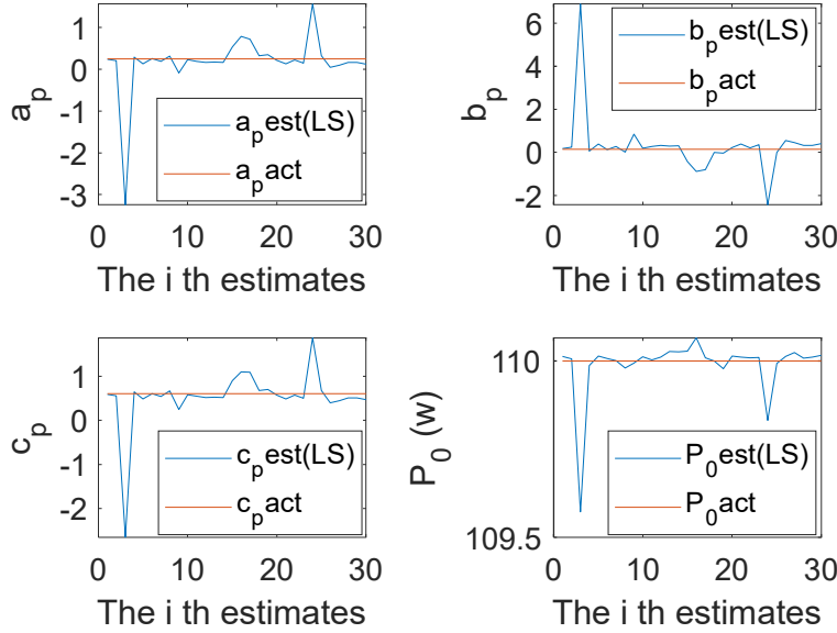
Fig. 2. The ZIP estimation results for a single load with measurement noise (blue: estimated values; red: actual values).
